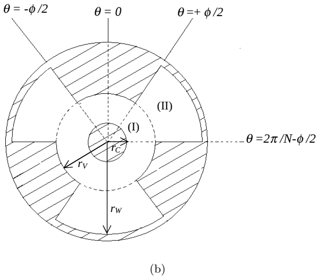
Figure 1. Cross section of a coaxial waveguide with ridged central conductor (configuration A) (a) and with vane-loaded outer conductor (configuration B) (b).
