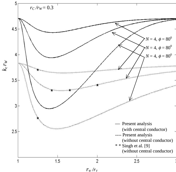
Figure 4. Variation of the eigenvalue of the typical waveguide mode TE_{0,1} with the ratio of the waveguide to ridge radii for configuration B , taking the vane dimensions as the parameters.
