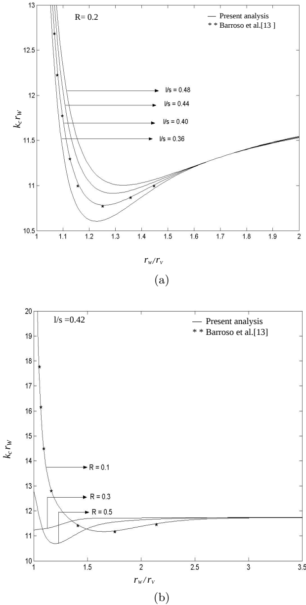
Figure 3. Variation of the eigenvalue of the typical waveguide mode TE_{6,2} with the ratio of the waveguide to ridge radii for configuration A, taking the slot width relative to the ridge periodicity (a) and the ridge depth relative to the outer ridge-edge radius (b) as the parameters.
