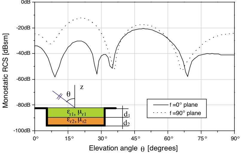
Figure 5. Monostatic RCS \sigma_{\theta\theta} for a \varphi -polarized incident plane wave at f = 10 GHz. The cavity dimensions are: 10\text{ cm} \times 10\text{ cm} \times 1.5\text{ cm} ; while the slab parameters are: d_1 = 1.02\text{ cm} , d_2 = 1.02\text{ cm} , \varepsilon_{r1} = 9.957 , \mu_{r1} = 0.037 , \varepsilon_{r2} = 5.747 , \mu_{r2xx} = \pm 0.283 , \mu_{r2yy} = -0.283 , \mu_{r2zz} = 0.283 .
