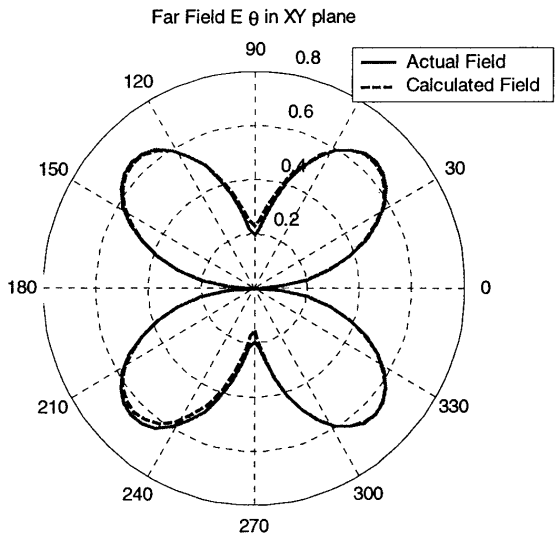
Figure 4. Comparison of E_\theta far field.
