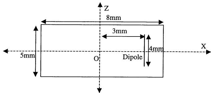
Figure 23. Dimensions of the dielectric resonator antenna.
