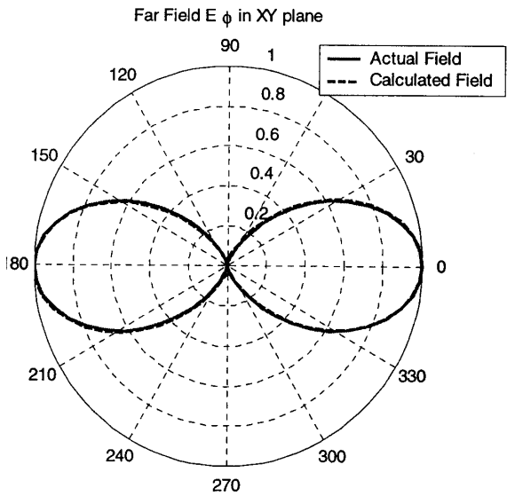
Figure 3. Comparison of E_\phi far field.
