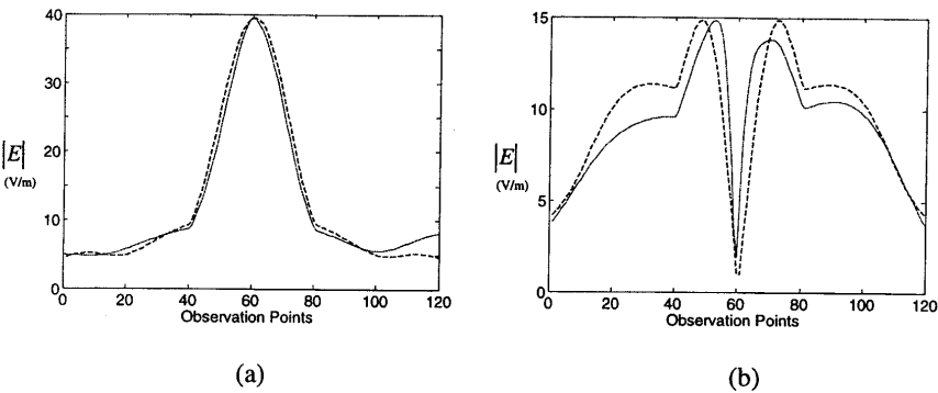
Figure 15. Near-field of circular waveguide antenna at 10 GHz, (solid line for equivalent dipoles and dashed lines for actual antenna) (a) E_y , (b) E_z .
