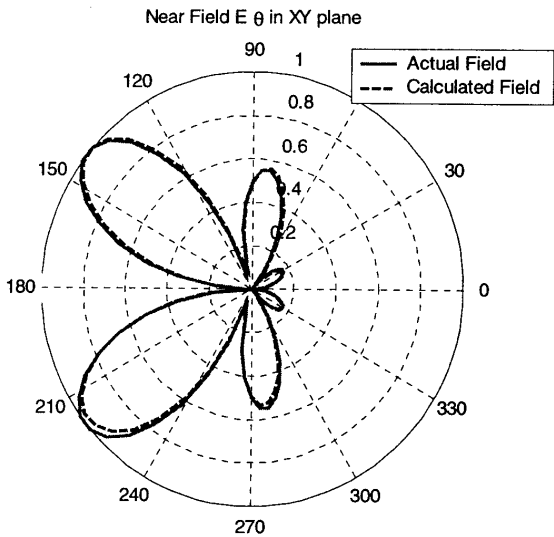
Figure 2. Comparison of E_\theta near field.
