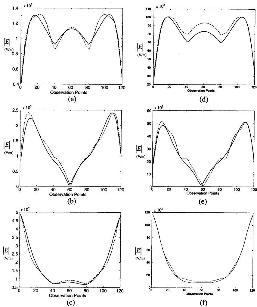
Figure 25. Near-field of the DRA and the equivalent dipoles at different frequencies, (solid line for equivalent dipoles and dashed lines for actual antenna) (a) E_x , (b) E_y , (c) E_z (7.5 GHz), (d) E_x , (e) E_y , (f) E_z (11 GHz).
