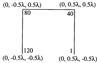
Figure 20. Coordinates of the near field plane cut for DRA.
