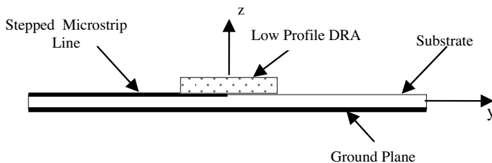
Figure 1. Low profile DRA with stepped microstrip feed.
