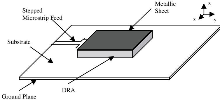
Figure 4. Compact DRA with metallic sheet covering the entire top surface.
