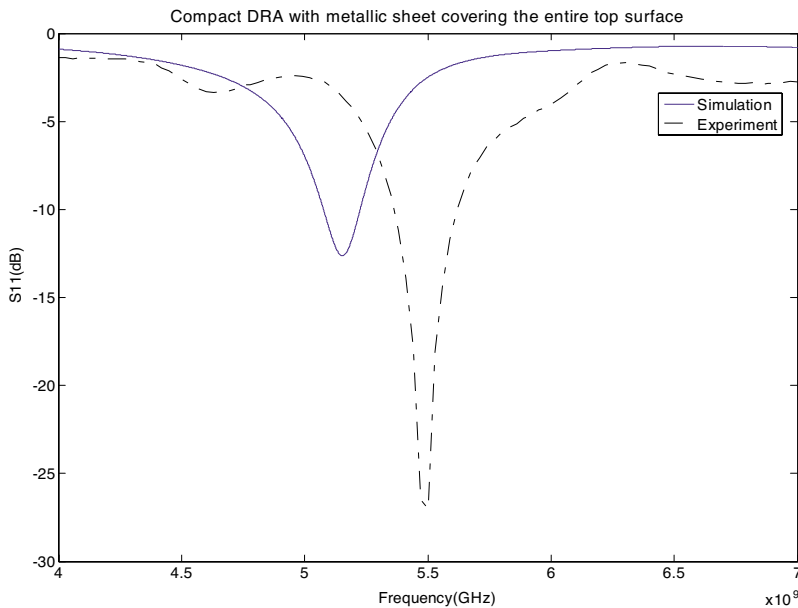
Figure 9. Computed and measured return loss vs. frequency for compact DRA with large metallic sheet.
