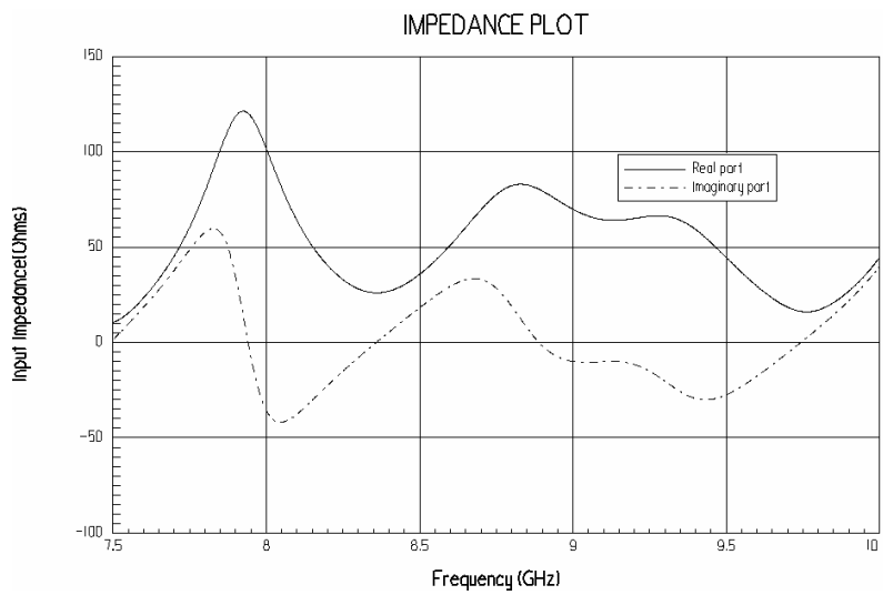
Figure 5. Computed input impedance, real and imaginary parts, vs. frequency.
