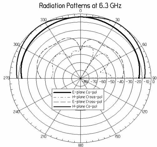
Figure 10. Computed radiation pattern at 6.3 GHz for compact DRA with small metallic sheet.
