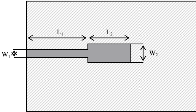
Figure 2. Top view of stepped microstrip feed line W_1 = 1.2 mm, W_2 = 3 mm, L_1 + L_2 = 45 mm.
