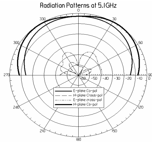
Figure 11. Computed radiation pattern at 5.1 GHz for compact DRA with large metallic sheet.
