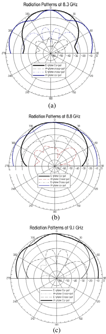
Figure 7. Computed radiation patterns at (a) 8.3 GHz, (b) 8.8 GHz and (c) 9.1 GHz for low profile DRA.
