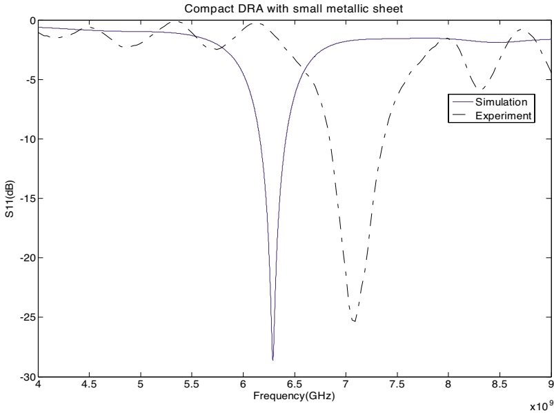
Figure 8. Computed and measured return loss vs. frequency for compact DRA with small metallic sheet.
