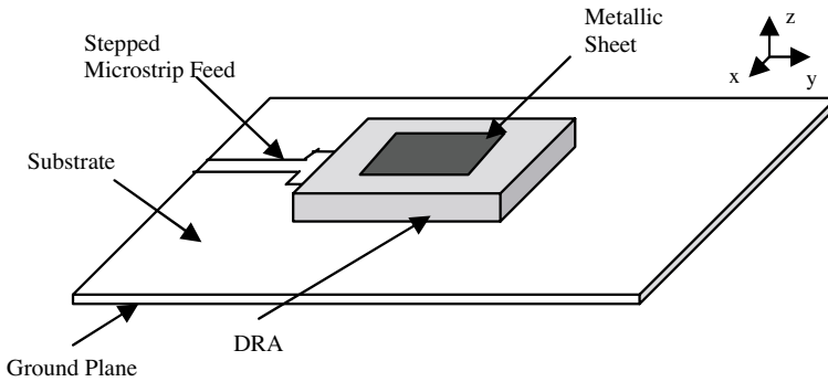
Figure 3. Geometry of compact DRA with small metallic sheet.
