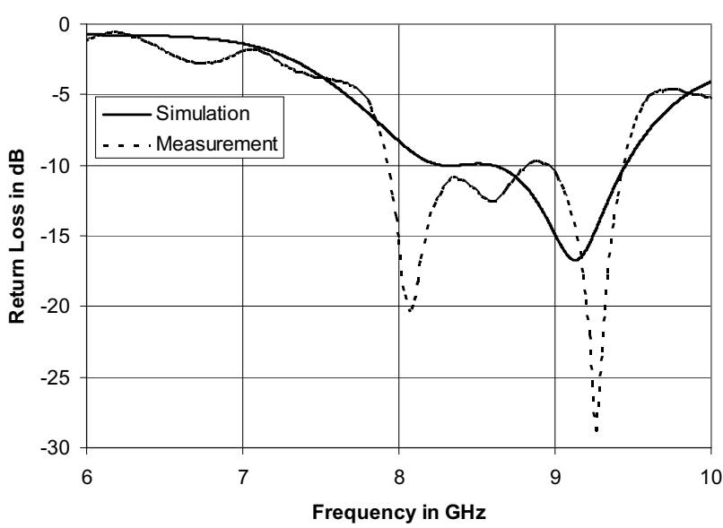
Figure 6. Computed and measured return loss vs. frequency for low profile DRA.
