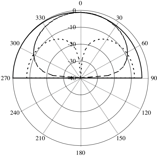
(a) 3 GHz
