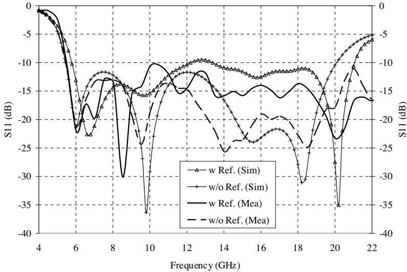
Figure 7. Measured and simulated return loss of the CPW fed slot antenna with and without reflector — without reflector (measurement), —+— without reflector (simulation), — with reflector (measurement), —△— with reflector (simulation).
