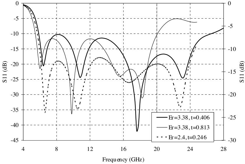
Figure 13. Simulated return loss with different dielectric substrate \epsilon_r = 3.38 , t = 0.406 mm, \epsilon_r = 3.38 , t = 0.813 mm.
