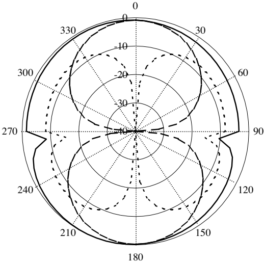
(c) 15 GHz
