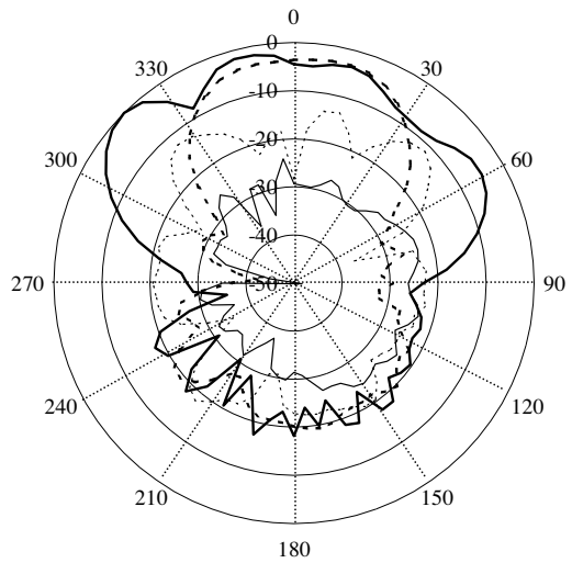
Figure 4. Measured radiation patter at 9 GHz (10 dB/Div) — E-Co, \cdots H-Co, --- E-X, ---- H-X.
