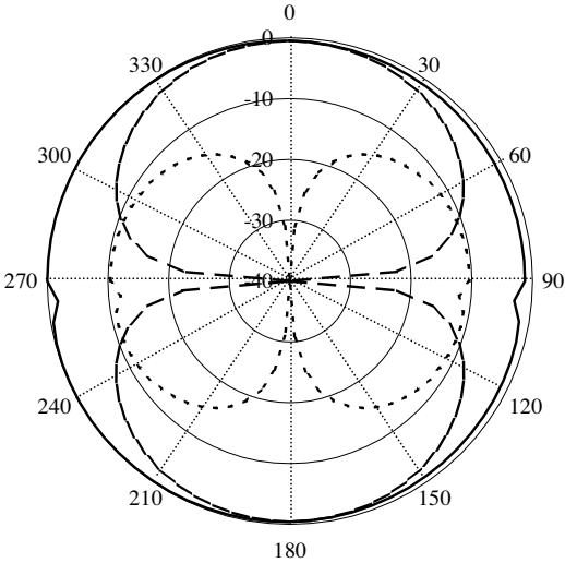
(a) 5 GHz
