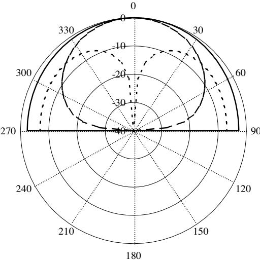
(c) 7 GHz
