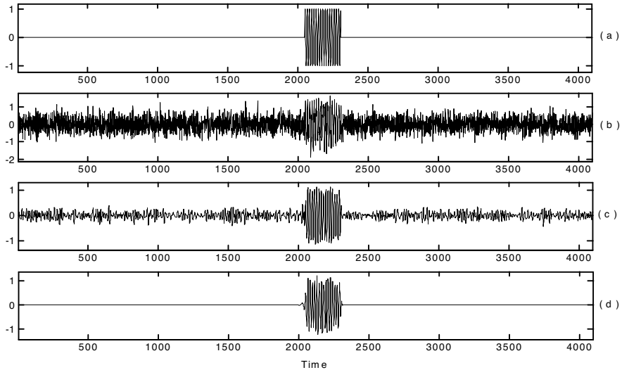
Figure 6. (a) The clean RF radar pulse x(n) (b) The received noisy RF radar pulse y(n) , \text{SNR} = -3 \text{ dB} (c) The result of the first stage (d) The result of the second stage.
