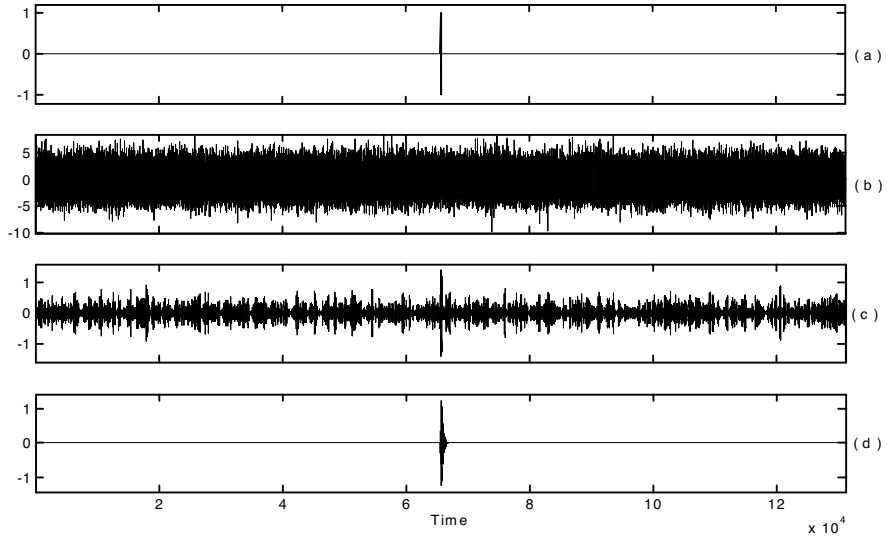
Figure 7. (a) Clean signal (b) Noisy signal SNR = -18 dB (c) denoised signal after the first stage (d) denoised signal after the second stage.
