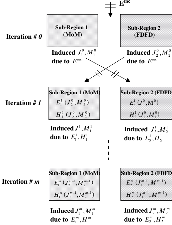
Figure 2. Scheme for the iterative procedure applied by converting the electric and magnetic currents to field components generated on the other region.
