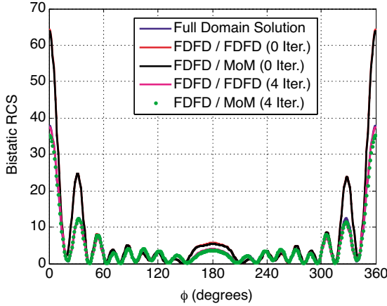
Figure 4. Bistatic echo width a conducting and dielectric cylinder excited by a TM_z plane wave incident at \phi^i = 180^\circ .
