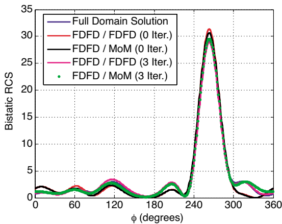
Figure 6. Bistatic echo width a conducting square and dielectric ellipsoid excited by a TM_z plane wave incident at \phi^i = 90^\circ .
