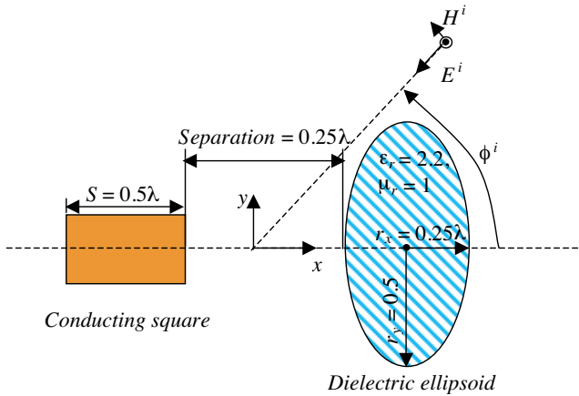
Figure 5. Geometry of a conducting square and a dielectric ellipsoid.
