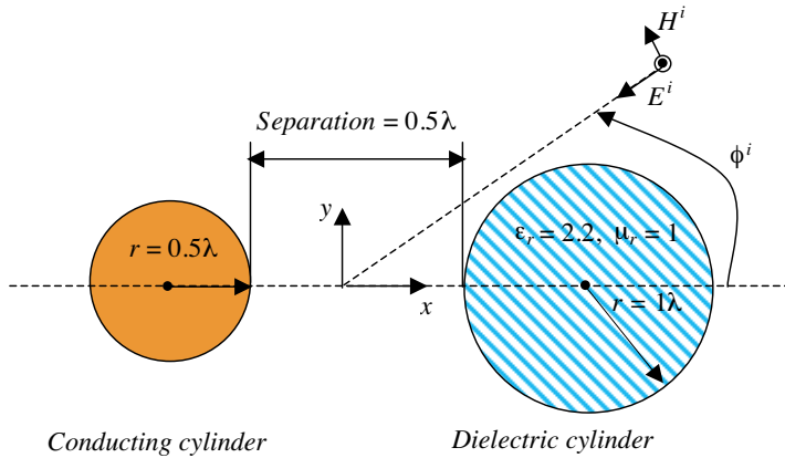
Figure 3. Geometry of one conducting and one dielectric cylinder.
