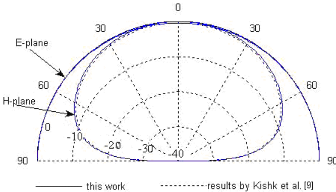
Figure 3. Radiation patterns (in dB) of DRAs with a = 2.975 cm, L = 5.0 cm, W = 0.06 cm, b = 6.49 , and f = 1.375 GHz. Solid line denotes patterns of hemispheroidal DRA ( b/a=1.001 ) of this work, and dash line denotes patterns of a hemispherical DRA [9].
