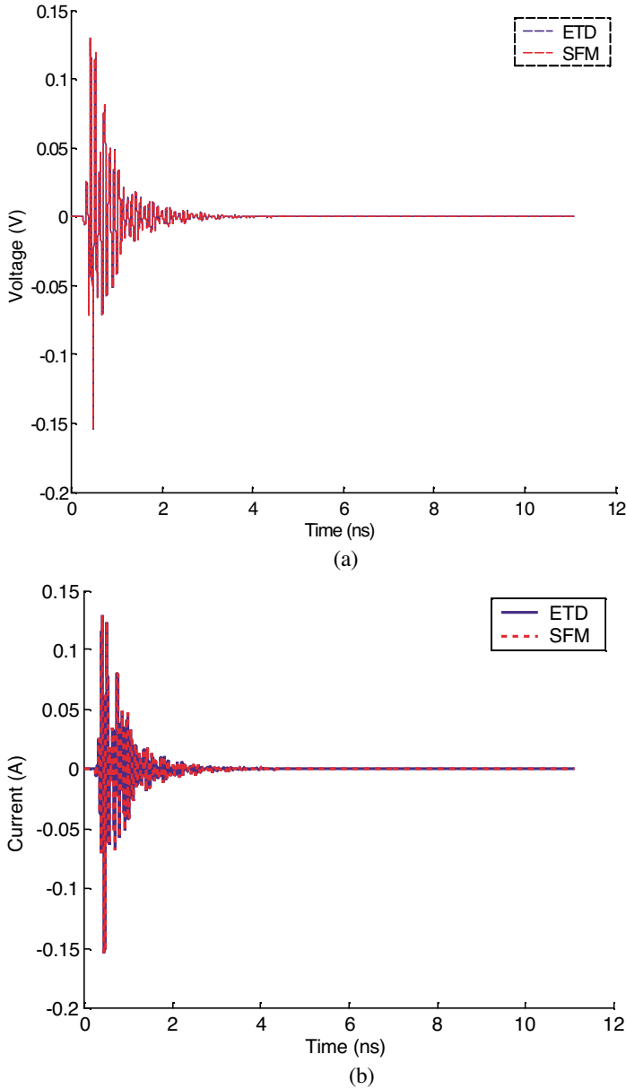
Figure 5. Time-domain response from the ETD algorithm and the SFM for an infinite rectangular DRA array with a 45° scan angle: (a) sampled voltage and (b) sampled current.
