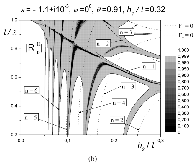
Figure 3. Reflection coefficient behavior in the H -polarization case ( \text{Re}\varepsilon < -1 ).
