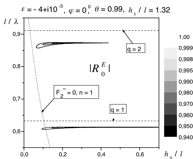
Figure 6. Behavior of the reflection coefficient in the E -polarization case ( \text{Re}\varepsilon < -1 ).
