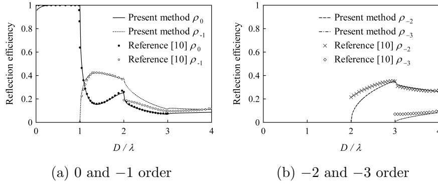
Figure 5. Diffraction efficiency as functions of D/\lambda (E-wave). N = 25 , Q = 25 , n_U = 1 , H = 0.25\lambda , and \theta = 0^\circ .
