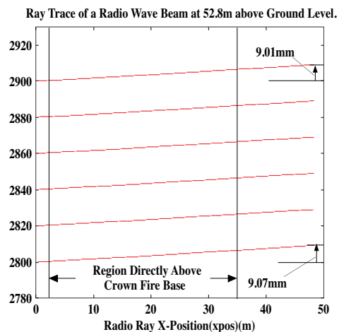
Figure 13. 3000 MHz ray trace at 52.8 m above ground level.
