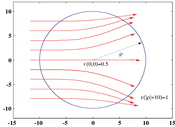
Figure 4. Rays (excluding rays at edges) refraction in a dielectric pothole.
