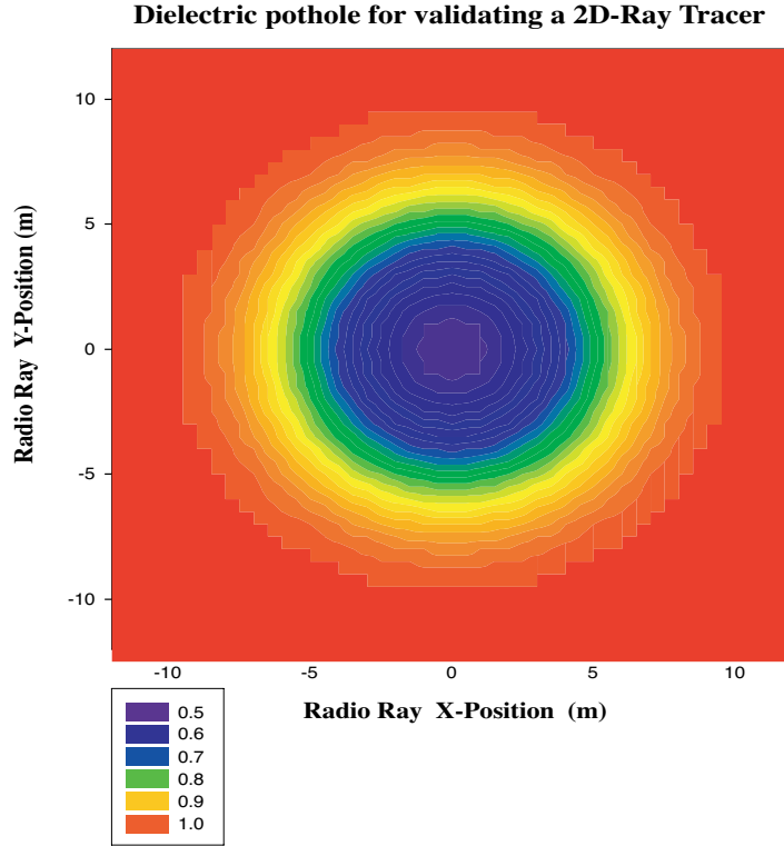
Figure 3. Dielectric pothole used in the validation of the 2D ray tracing scheme.
