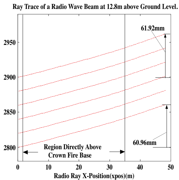
Figure 8. 450 MHz ray trace at 12.8 m above ground level.
