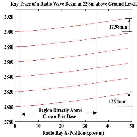
Figure 11. 1200 MHz ray trace at 22.8 m above ground level.
