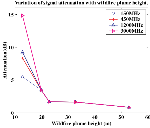
Figure 14. Signal attenuation due to refraction in a wildfire plume.
