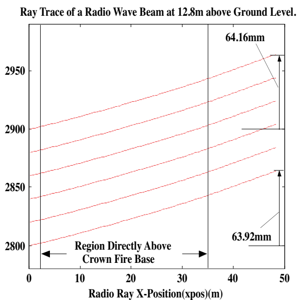
Figure 9. 3000 MHz ray trace at 12.8 m above ground level.
