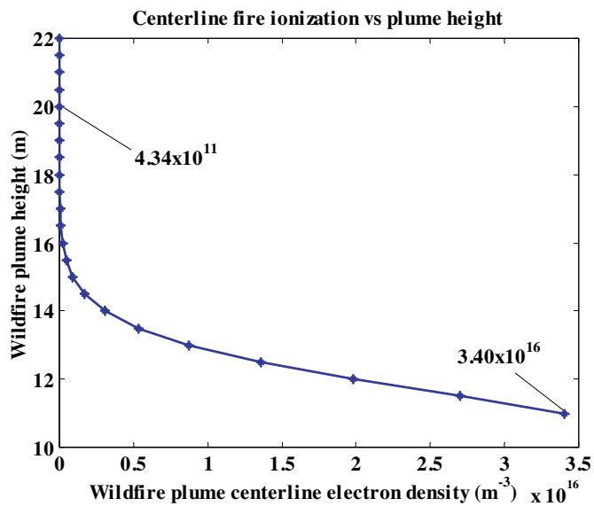
Figure 7. Centerline plume ionization variation with plume.
