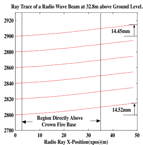
Figure 12. 900 MHz ray trace at 32.8 m above ground level.
