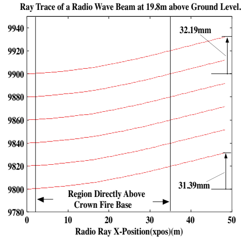
Figure 10. 150 MHz ray trace at 19.8 m above ground level.
