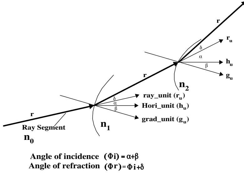
Figure 2. Ray trace through a non-homogeneous plume.
