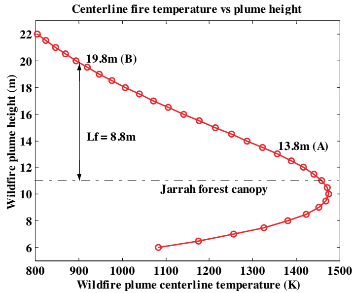
Figure 6. Centerline temperature variation with plume height is the region up to 22 m.
