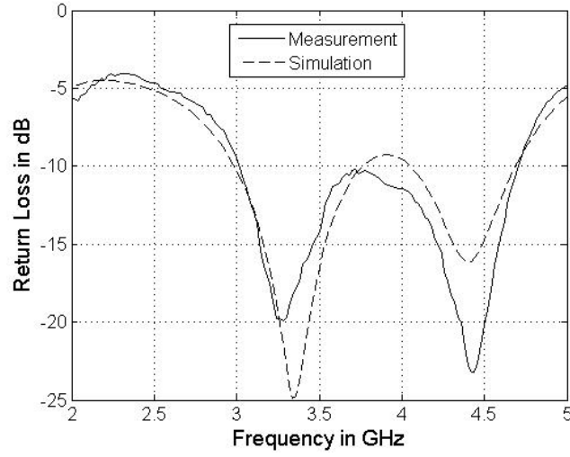
Figure 11. Measured and simulated return loss for the CPW-fed wide slot with V-shaped stubs.
