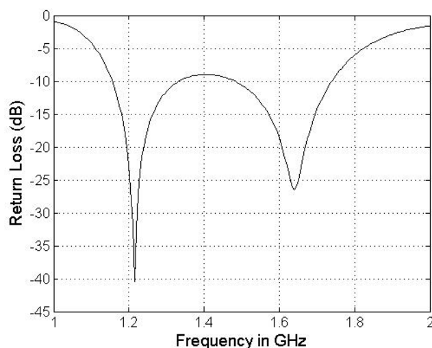
Figure 8. Return loss for CPW-Fed wide slot with inverted F-shaped stub.
