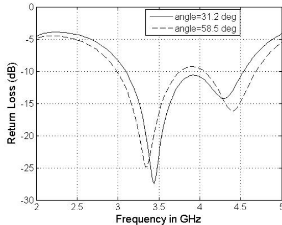
Figure 6. Return Loss for the CPW-Fed wide slot with V-shaped stubs.
