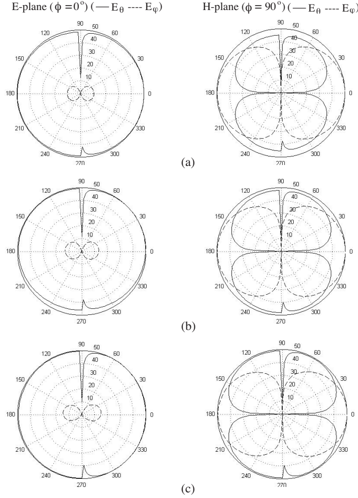
Figure 7. E -plane and H -plane radiation patterns for the antenna with wide angle ( 58.5^\circ ) V-shaped stubs, (a) Frequency=3 GHz, (b) Frequency=3.5 GHz, (c) Frequency=4.5 GHz.
