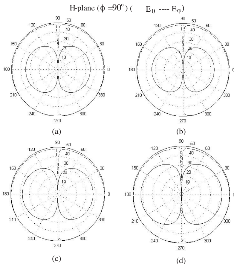
Figure 10. H -plane ( \phi = 90^\circ ) radiation patterns for wide slot with inverted F-shaped stub, (a) Frequency=1.2 GHz, (b) Frequency=1.5 GHz, (c) Frequency=1.35 GHz, (d) Frequency=1.65 GHz.
