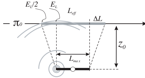
Figure 4. Geometry for the definition of the antenna effective footprint L_{eff} on \pi_0 according to a spherical radiation model from the antenna edges. E_L is the field amplitude on \pi_0 at the projections of the antenna boundary.
