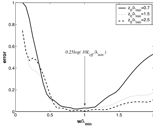
Figure 7. CRH antenna: reconstruction r.m.s. error \varepsilon(E_{0,y}, \sum_{m,n} v_{y,mn} h_{mn,y}) , at time t = 0.75 ns vs. the scaling factor w_x = w_y = w for different distances z_0 of the observation plane to the antenna and therefore of the effective antenna footprint L_{eff} on \pi_0 . In this case \lambda_{\min} = 3 cm.
