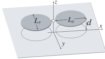
Figure 12. Agrawal dipole: geometry size: L_x = 5 \text{ cm} , L_y = 4.6 \text{ cm} , d = 2.4 \text{ cm} . Reflecting panel size: 20 \times 20 \text{ cm}^2 .
