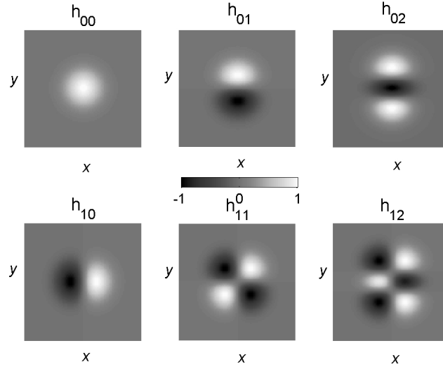
Figure 2. Some two-dimensional Associate Hermite functions having equal scaling factors w_x = w_y .
