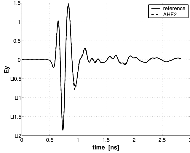
Figure 9. CRH antenna: interpolation of the near-field (in normalized units) on the \pi_0 plane at point x_0 = y_0 = 4.5 cm by the two-dimensional Associate Hermite series E_y(x_0, y_0, t) = \sum v_{y,mn}(t)h_{mn}(x, y, w) with N = M = 7 .
