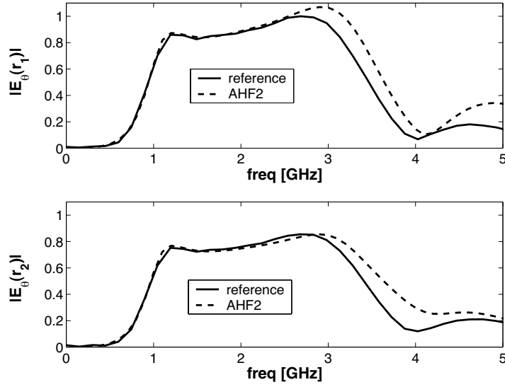
Figure 16. Agrawall dipole: comparison between reference solution and AHF2 reconstructions for the far field r|E_\theta| at angles (\theta = 0^\circ, \phi = 0^\circ) -up- and (\theta = 12^\circ, \phi = 0^\circ) -down-. Data in normalized units.
