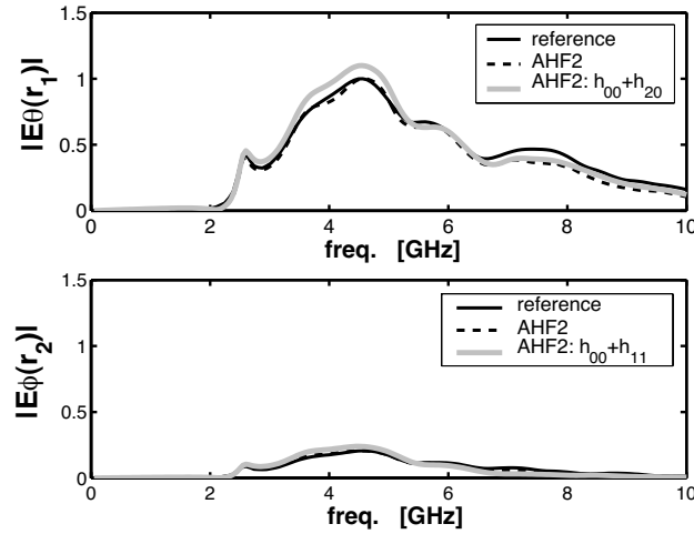
Figure 11. CRH antenna: comparison between reference solution and AHF2 reconstructions for the far-field data (normalized units) at the boresight, P_1 = (r_1 = 15 \text{ cm}, \theta = 0^\circ, \phi = 0^\circ) , and off-the-boresight, P_2 = (r_2 = 48.8 \text{ cm}, \theta = 18^\circ, \phi = 45^\circ) .
