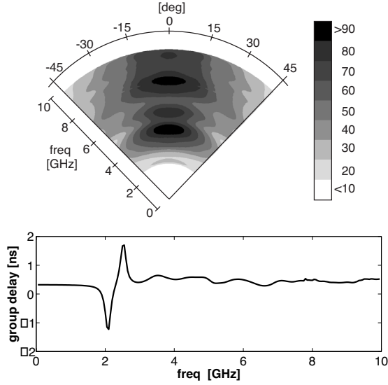
Figure 10. CRH antenna: transfer function (in normalized units) at \phi = 0^\circ , amplitude of the \theta -component and group delay along the boresight.
