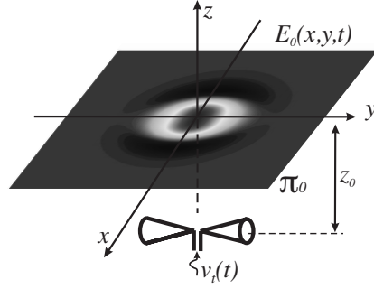
Figure 1. The relevant geometry for the Hermite processing of a time-varying near field.
