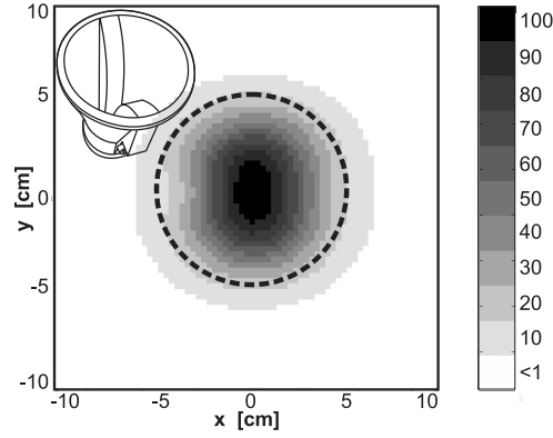
Figure 6. Normalized energy e(x, y) = \|\mathbf{E}(\cdot, t)\|_2 radiated by the circular ridged horn on the plane \pi_0 placed at distance z_0 = 2.1 cm from the antenna aperture. The circle indicates the antenna rim projection over \pi_0 .
