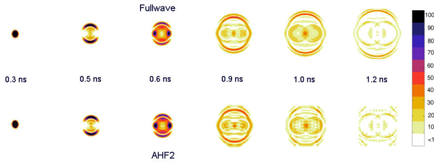
Figure 15. Agrawall dipole: some snapshots of the near field ( |E_x(x, y, t)| component) on the observation plane \pi_0 placed at a distance z_0 = 18 mm from the antenna as computed by FDTD (upper line) and interpolated by AHF2s (lower line).
