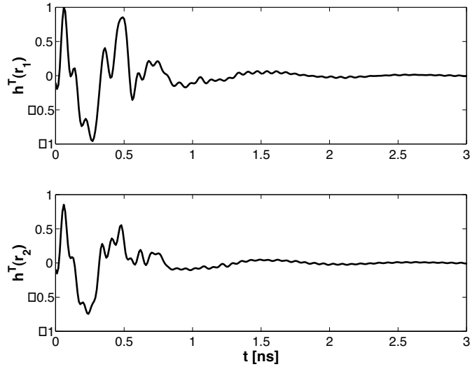
Figure 17. Agrawall dipole: time-domain effective height (in normalized units) at angles (\theta = 0^\circ, \phi = 0^\circ) -up- and (\theta = 12^\circ, \phi = 0^\circ) -down- as computed by AHF2 processing.
