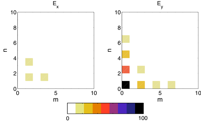
Figure 8. CRH antenna: energy spectrum of the Hermite coefficients for the field interpolation on \pi_0 .
