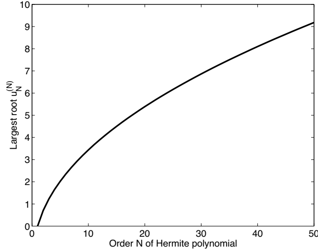
Figure 5. Largest roots u_N^{(N)} of the Hermite polynomials H_N(u) .
