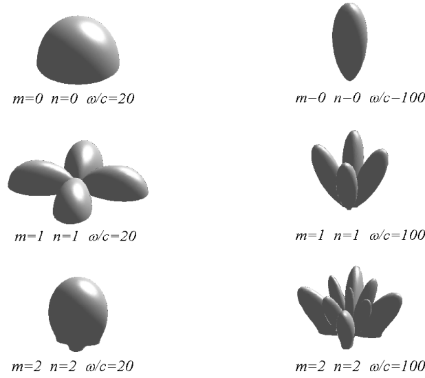
Figure 3. Examples of the k -domain AHF2 functions |h_{mn}(-\frac{k_x}{2\pi}, -\frac{k_y}{2\pi}, \frac{1}{2\pi w_x}, \frac{1}{2\pi w_y})| of different orders plotted at some frequencies in angular coordinates (\theta, \phi) .
