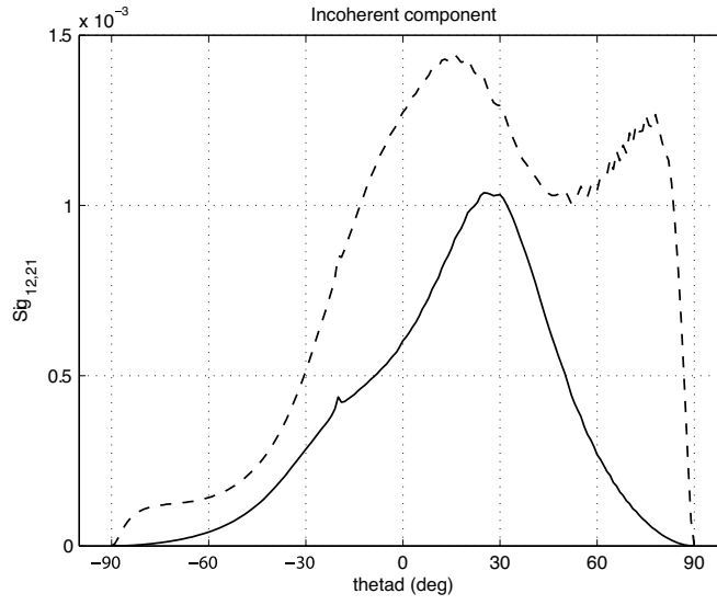
Figure 23. Same characteristics as the previous figure. Incoherent component VH (dashed line), HV (solid line).
