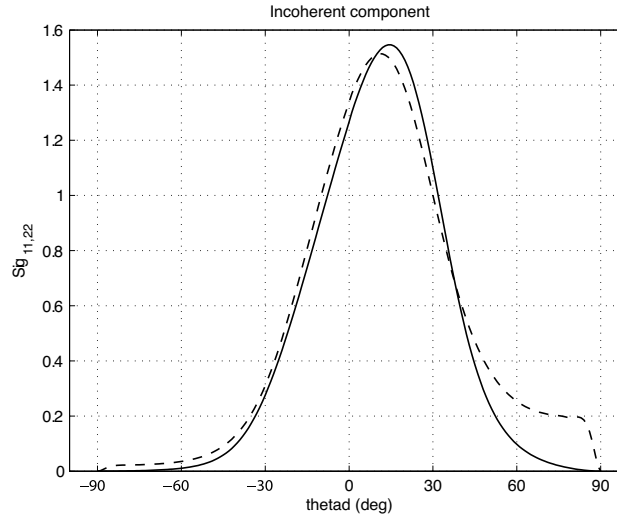
Figure 22. Incoherent components \gamma^{incoh}(\theta_d) to the order 2. VV (dashed line), HH (solid line), Surface height \sigma = 0.3/K_0 , correlation length l = 3/K_0 , slab thickness 500 nm. Permittivities \epsilon_0 = 1 , \epsilon_1 = 2.6896 + i0.0075 , \epsilon_2 = -40 - i1.1 . Incident angles: \theta_i = 20^\circ , \phi_i = 0^\circ , wavelength \lambda = 632.8 nm.
