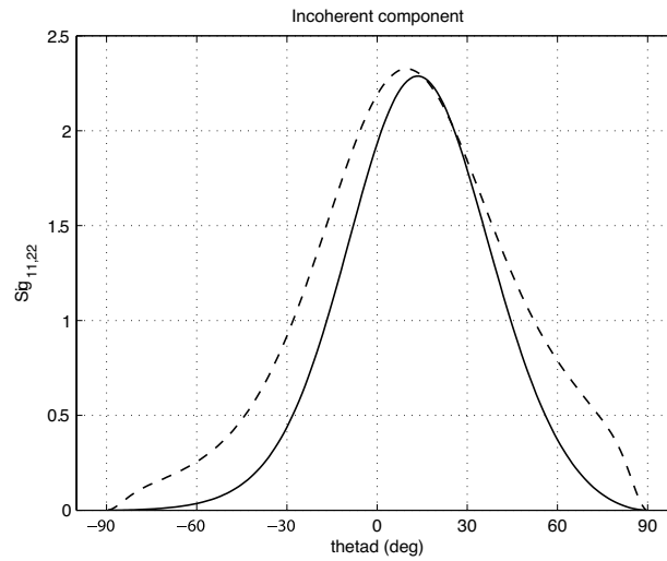
Figure 6. Incoherent components \gamma^{incoh}(\theta_d) in the order 2 approximation as a function of the scattering angle \theta_d . VV (dashed line), HH (solid line). Incident wavelength \lambda = 632.8\text{ nm} , height \sigma = 0.3/K_0 , correlation length l = 3/K_0 . Angles: \theta_i = 20^\circ , \phi_i = 0^\circ , permittivity: \epsilon_0 = 1 , \epsilon_1 = -40 - i1.1 .
