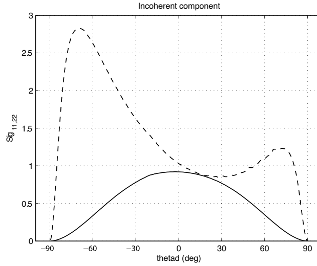
Figure 9. Incoherent components \gamma^{incoh}(\theta_d) in the order 2 approximation as a function of the scattering angle \theta_d . VV (dashed line), HH (solid line), Incident wavelength \lambda = 632.8 nm, surface height \sigma = 1/K_0 , correlation length: l = 1/K_0 . Angles: \theta_i = 20^\circ , \phi_i = \phi = 0^\circ . Permittivity: \epsilon_0 = 1 , \epsilon_1 = -40 - i 1.1 .
