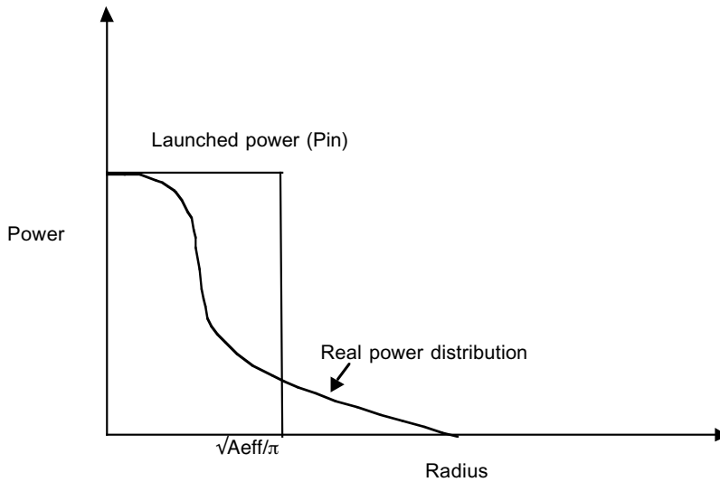
Figure 4. Definition of effective core area.
