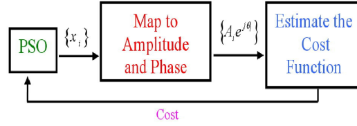
Figure 5. Block diagram representation of the linear array synthesis problem. Here the particles are x_i \in \{0 \leq x_i \leq 1, i = 1, 2, \dots, 2N\} . Amplitudes and phases are ranged as A_i \in \{A_{\min} \leq A_i \leq A_{\max}, i = 1, 2, \dots, N\} and \theta_i \in \{0 \leq \theta_i \leq 2\pi, i = 1, 2, \dots, N\} , respectively.
