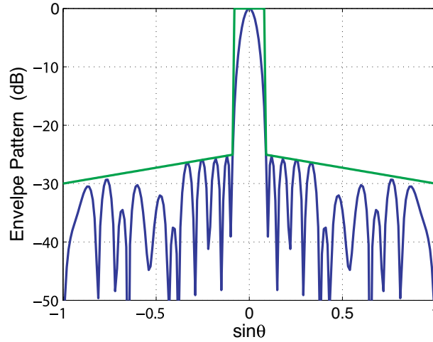
Figure 7. Radiation pattern of the linear array antenna corresponding to best case of Figure 6 ( T_0 = 0.05 ).
