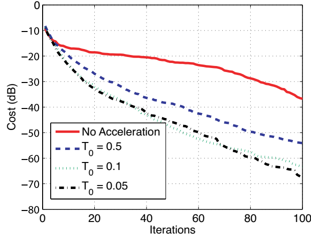
Figure 6. Convergence curves for the synthesis of symmetric pattern by using a linear array of 14 elements. The population size is 8 particles. The inertia factor w is decreased linearly from 0.9 to 0.2. c_1 = c_2 = 2.0 .
