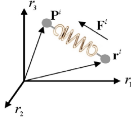
Figure 1. A 3-D illustration of the mechanical analogy to the PSO. The i th particle will experience a mechanical force identical to a spring with one end attached to the position and the other end attached to the particle's itself.
