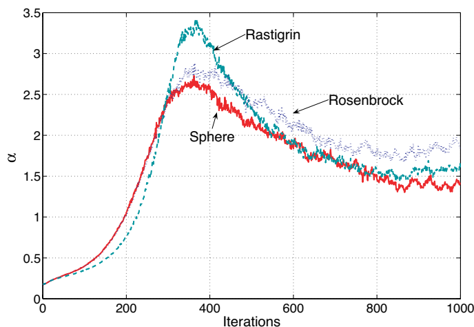
Figure 3. The time evolution of the \alpha -index for the problem of Figure 2. The PSO algorithm was run 1000 times and averaged results are reported.
