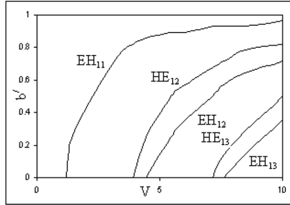
Figure 7. Dispersion curves ( b' Vs V graphs) for odd guided modes when e = 0.8 .
