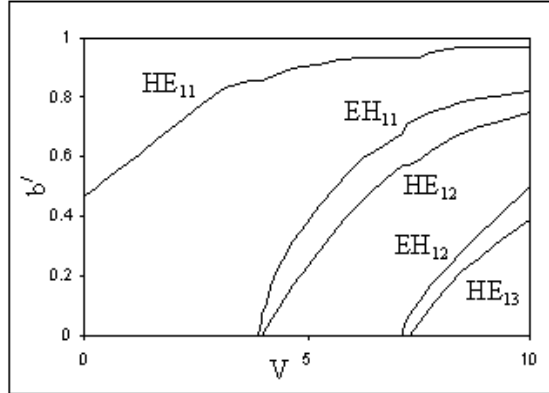
Figure 2. Dispersion curves ( b' Vs V graphs) for even guided modes when e = 0.4 .
