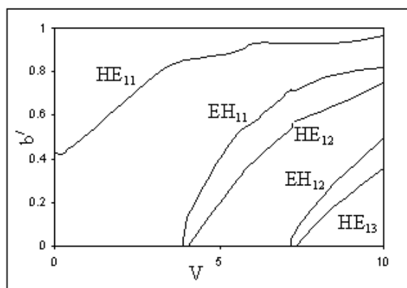
Figure 4. Dispersion curves ( b' Vs V graphs) for even guided modes when e = 0.8 .
