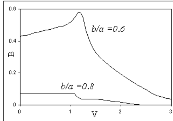
Figure 8. The dependence of the normalized modal birefringence B on the normalized frequency parameters V for \frac{b}{a} = 0.6 and for \frac{b}{a} = 0.8 .
