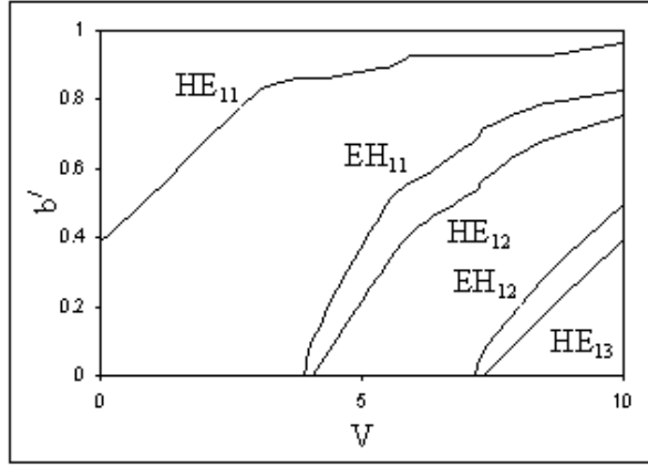
Figure 6. Dispersion curves ( b' Vs V graphs) for odd guided modes when e = 0.6 .
