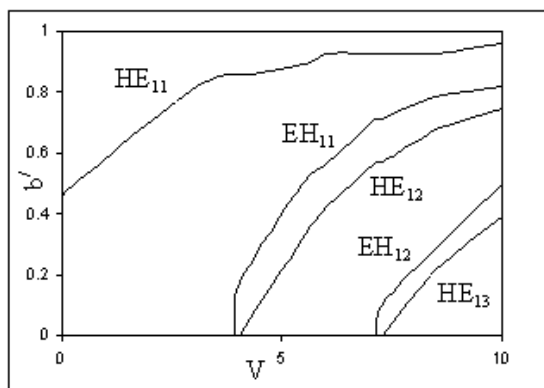
Figure 3. Dispersion curves ( b' Vs V graphs) for even guided modes when e = 0.6 .
