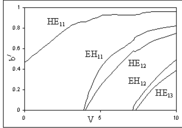
Figure 5. Dispersion curves ( b' Vs V graphs) for odd guided modes when e = 0.4 .
