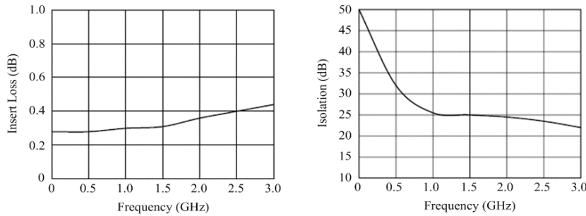
Figure 2. Insert loss and isolation of SPDT switch.
