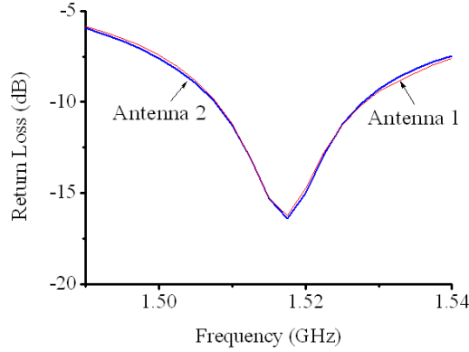
Figure 3. Measured return losses of antenna 1 and antenna 2.
