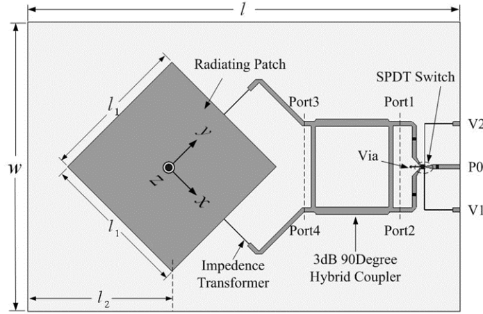
Figure 1. Configuration of the square microstrip patch antenna with switchable polarization and a coordinate system. l = 180 mm, w = 120 mm, l_1 = 61.34 mm, l_2 = 70 mm.
