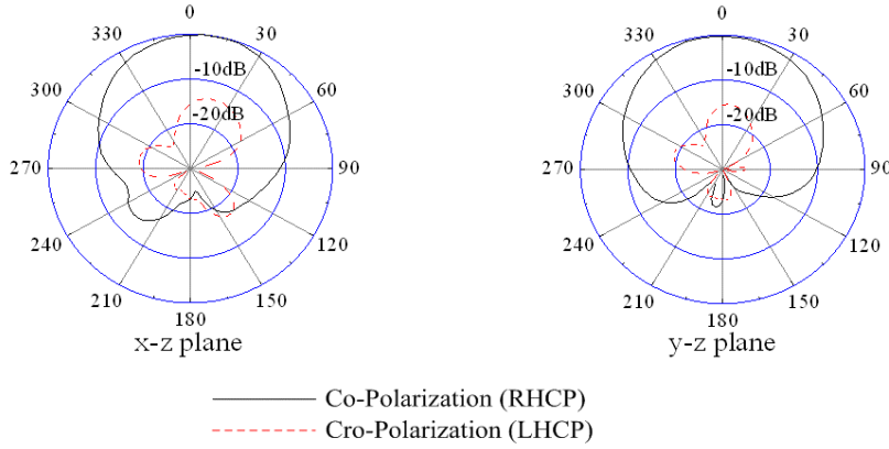
Figure 4. Measured radiation patterns in x - z plane and y - z plane for antenna 1 at 1.5175 GHz.
