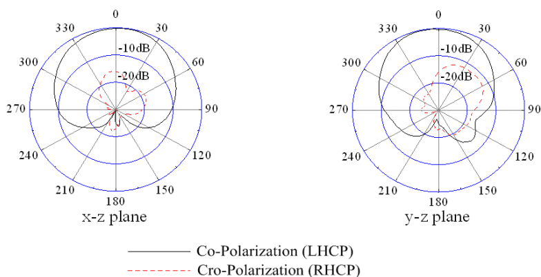
Figure 5. Measured radiation patterns in x - z plane and y - z plane for antenna 2 at 1.5175 GHz.
