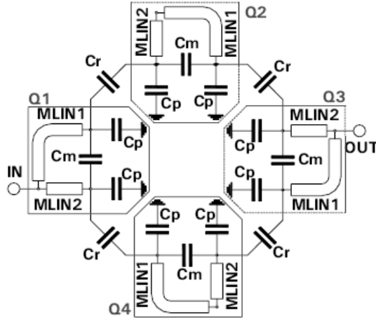
Figure 2. Circuit simulator scheme.
