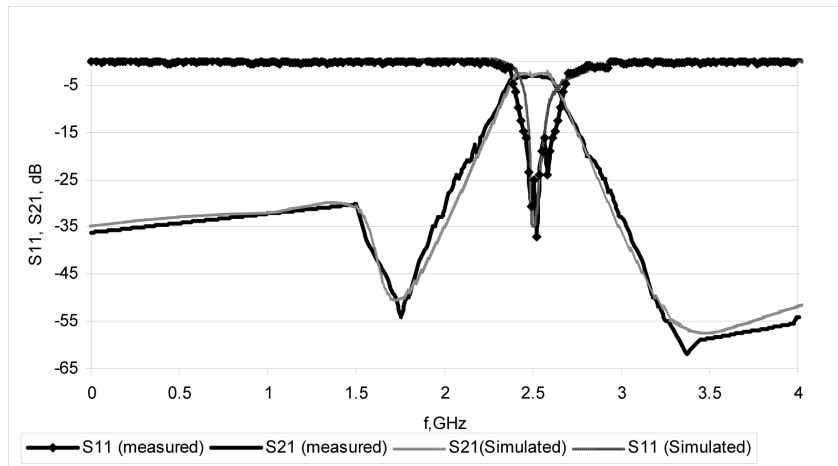
Figure 4. Simulated and measured S_{11} and S_{21} parameters of the filter.
