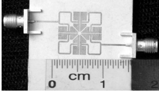
Figure 3. Photograph of the realised filter.
