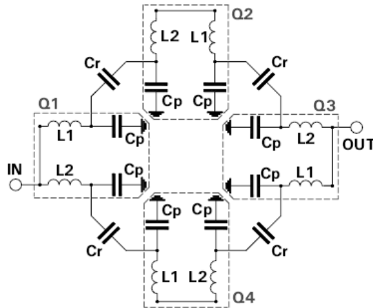
Figure 1. Basic electric scheme of proposed filter.
