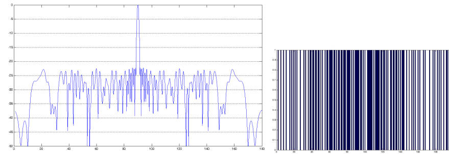
Figure 7. Far-field pattern (left) and element configuration (right) of result no. 3. “on” elements are shown with dark lines.
