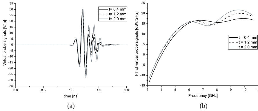
Figure 4. The signals received by the virtual probes at \theta = 90^\circ , \varphi = 0^\circ (substrate permittivity as 3.0): (a) time domain, (b) Frequency domain.
