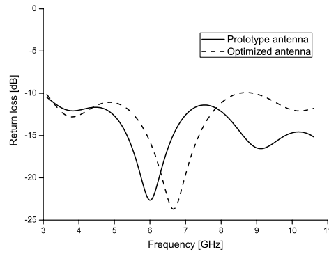
Figure 6. Simulated return loss of the prototype antenna and the optimized antenna.
