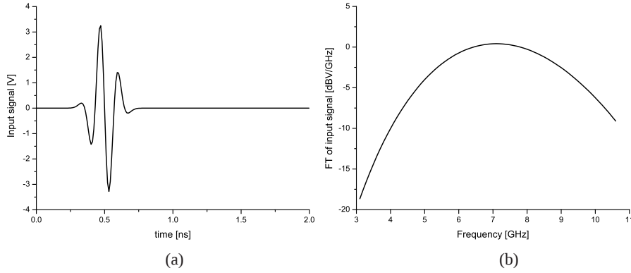
Figure 2. Antenna input signal: (a) time domain, (b) frequency domain.
