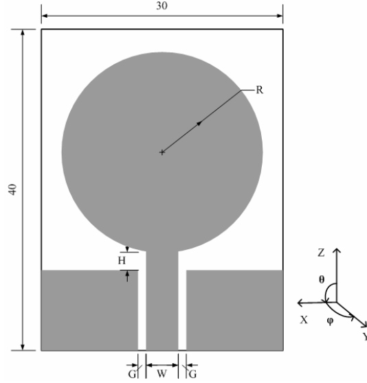
Figure 1. Geometry of prototype antenna and the coordinate system (dimensions in mm).
