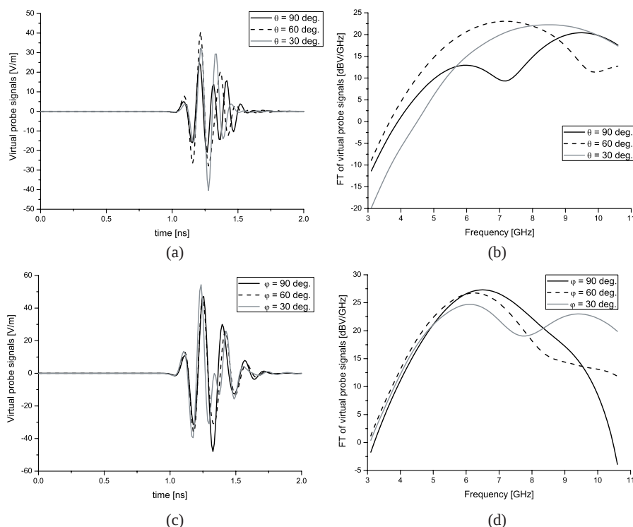
Figure 3. The received signals by the virtual probes of the prototype antenna: (a) time domain (X-Z plane), (b) frequency domain (X-Z plane), (c) time domain (X-Y plane), (d) frequency domain (X-Y plane).
