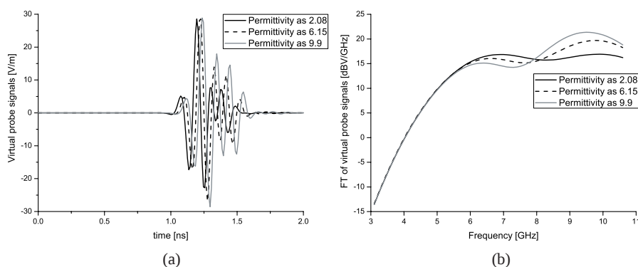
Figure 5. The signals received by the virtual probes at \theta = 90^\circ , \varphi = 0^\circ (substrate thickness as 0.4 mm): (a) time domain, (b) Frequency domain.
