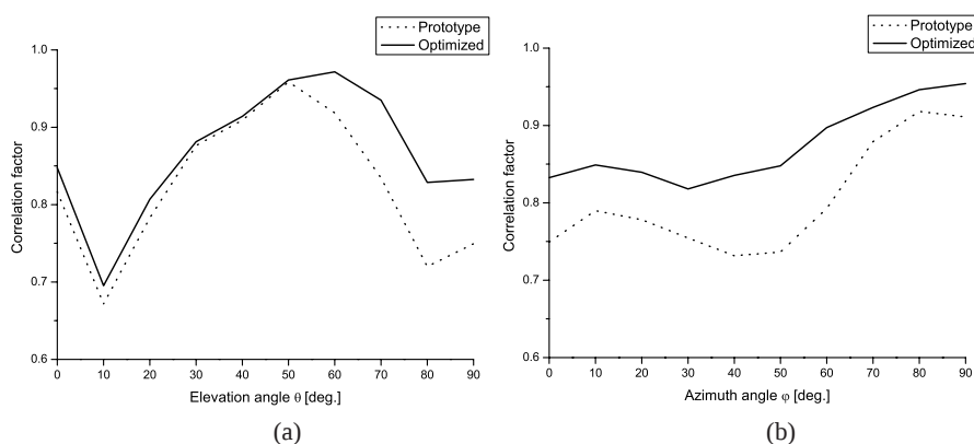
Figure 8. Correlation factors of the prototype antenna and optimized antenna: (a) X-Z plane, (b) X-Y plane.
