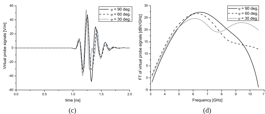
Figure 7. The received signals by the virtual probes of the optimized antenna: (a) time domain (X-Z plane), (b) frequency domain (X-Z plane), (c) time domain (X-Y plane), (d) frequency domain (X-Y plane).
