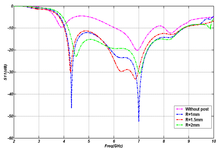
Figure 5. Return Loss of the antenna for various diameters of the posts. W1 = 22 mm, W2 = 11.5 mm, P = 5 mm, H = 8 mm, X = 5.7 mm, X1 = 4.5 mm, X2 = 2 mm, Y1 = 4 mm, Y2 = 8 mm.
