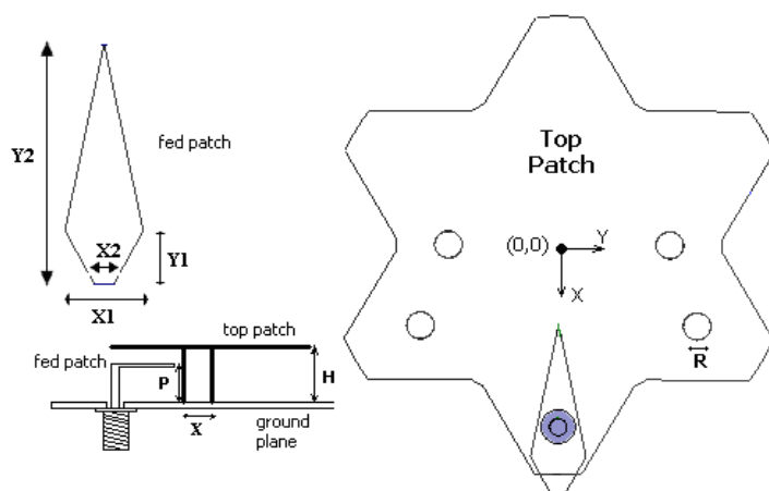
Figure 2. Geometry of proposed antenna with the diamond shaped feed patch.
