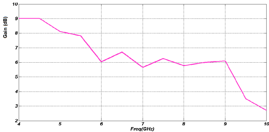
Figure 8. Gain of the proposed antenna at various frequencies.
