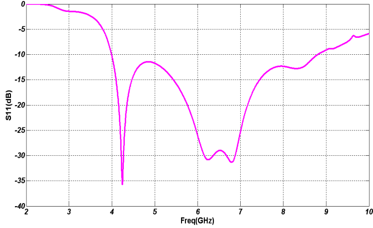
Figure 3. Return loss of the proposed antenna. W1 = 22 mm, W2 = 11.5 mm, P = 5 mm, H = 8 mm, X = 5.7 mm, X1 = 4.5 mm, X2 = 2 mm, Y1 = 4 mm, Y2 = 8 mm and R = 1.5 mm.
