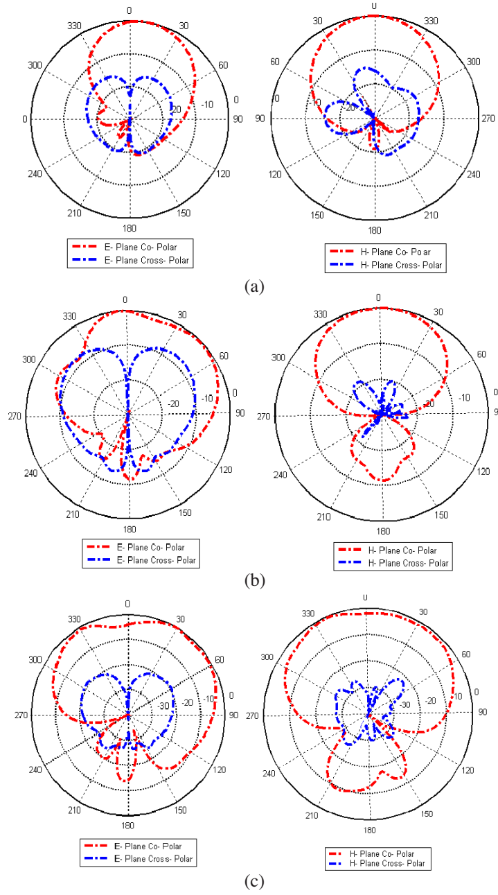
Figure 7. E & H-plane radiation pattern (a) at 4 GHz, (b) at 6 GHz, (c) at 8 GHz.
