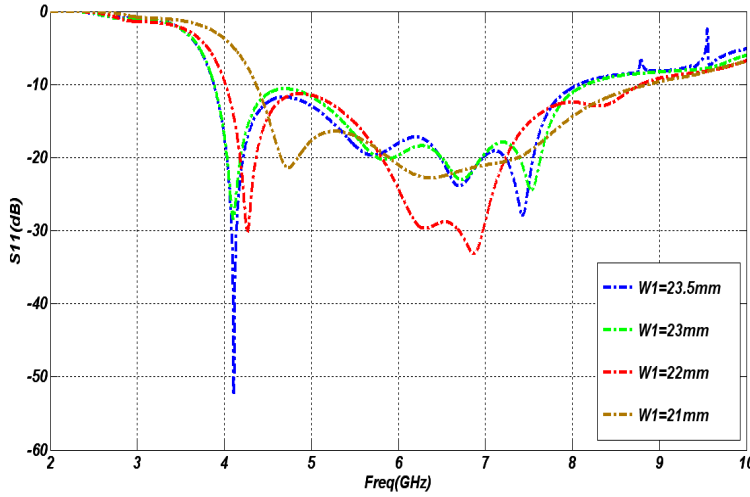
Figure 4. The Return loss of the antenna for various values of patch diameter, W1 . W2 = 11.5 mm, P = 5 mm, H = 8 mm, X = 5.7 mm, X1 = 4.5 mm, X2 = 2 mm, Y1 = 4 mm, Y2 = 8 mm and R = 1.5 mm.
