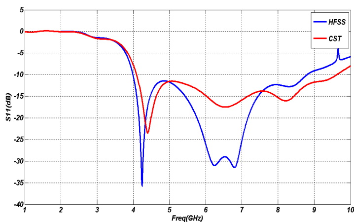
Figure 6. Comparison of the S_{11} obtained through HFSS and CST. W1 = 22 mm, W2 = 11.5 mm, P = 5 mm, H = 8 mm, X = 5.7 mm, X1 = 4.5 mm, X2 = 2 mm, Y1 = 4 mm, Y2 = 8 mm and R = 1.5 mm.
