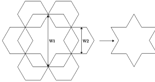
Figure 1. Process of building the star shaped patch antenna.
