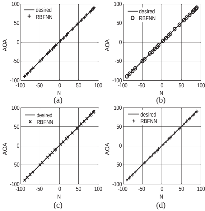
Figure 7. DOA estimates versus number of samples N for tripole array. Incident Source (1) \theta is varied from -90^\circ to 90^\circ and \varphi = 0^\circ .
