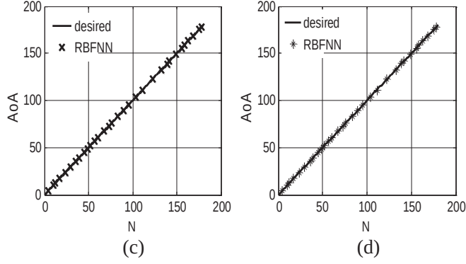
Figure 6. DOA estimates versus number of samples N for cross-dipole array. 8-Uncorrelated sources used with ( \Delta\varphi = 3^\circ ). Source (1) \varphi is varied from 0^\circ to 180^\circ and \theta = 90^\circ .
