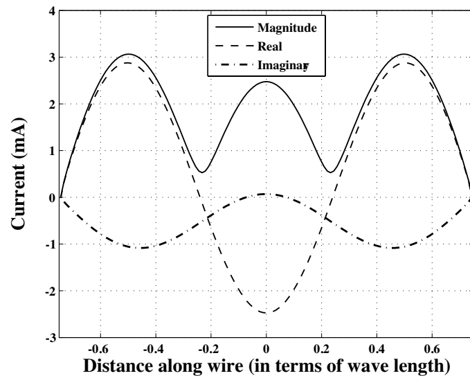
Figure 4. Current distribution along the thin wire of length \frac{3}{2}\lambda for \alpha = \frac{\pi}{2} .
