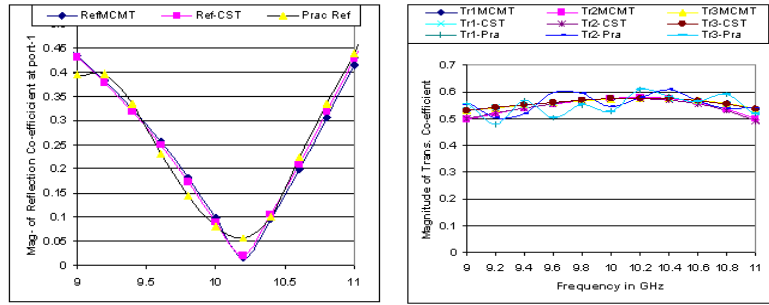
Figure 3. Comparison of theoretical, CST Microwave Studio simulated and measured data for an H -plane 1:3 WR-90 waveguide power divider with 2t = 19.5 mm.
