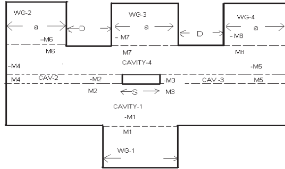
Figure 2. Cavity modeling and details of a basic 1:3 power divider.
