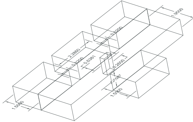
Figure 1. Three dimensional view of an H -plane 1:3 power divider, all dimensions are in cm.
