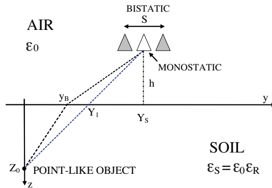
Figure 1. Snell approximation for incident beam at the interface between air-soil layers for the monostatic case.
