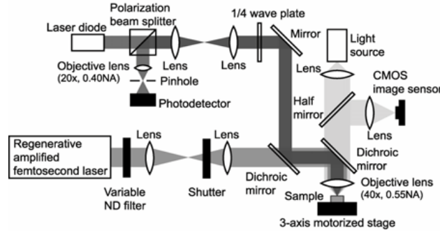
Figure 3. Experimental setup.
