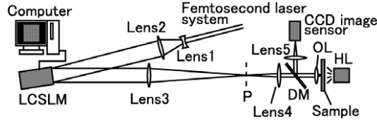
Figure 5. Experimental setup.
