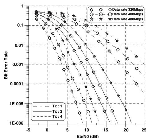
Figure 3. The BER performance of 1, 2 and 4 transmit antennas at data rate 320, 400 and 480 Mbps.
