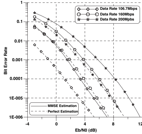
Figure 2. The BER performance of perfect channel estimation and MMSE method at the 2-transmit-antenna system.
