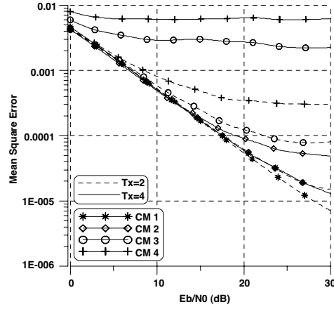
Figure 1. The MSE performance of proposed preambles applied to 2 and 4 transmit antennas with MMSE estimator.
