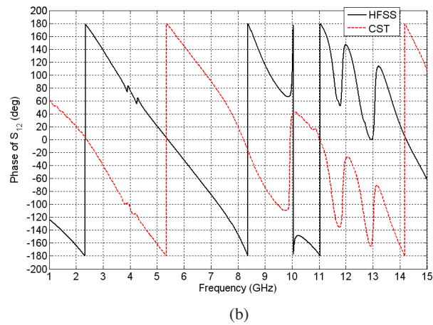
Figure 3. Phase of S_{12} (a) filter1, (b) filter2.
