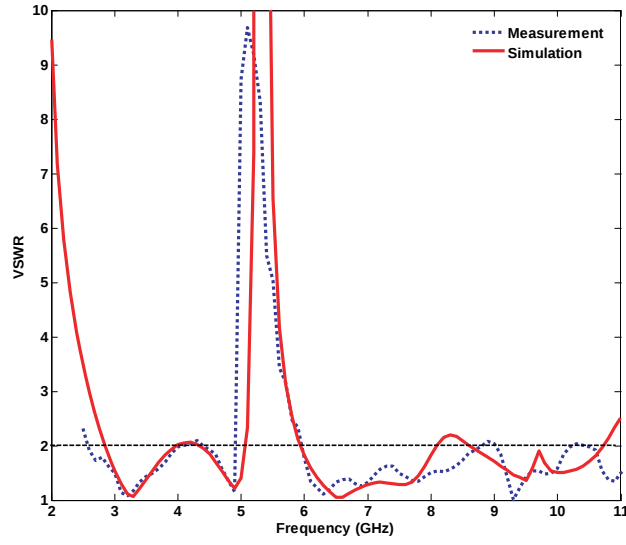
Figure 4. Simulated and measured VSWR of proposed antenna with dimensions of Table 1.
