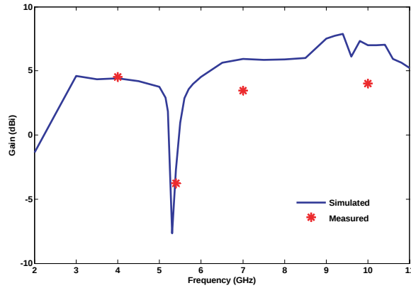
Figure 7. Simulated and measured gain of the proposed antenna.
