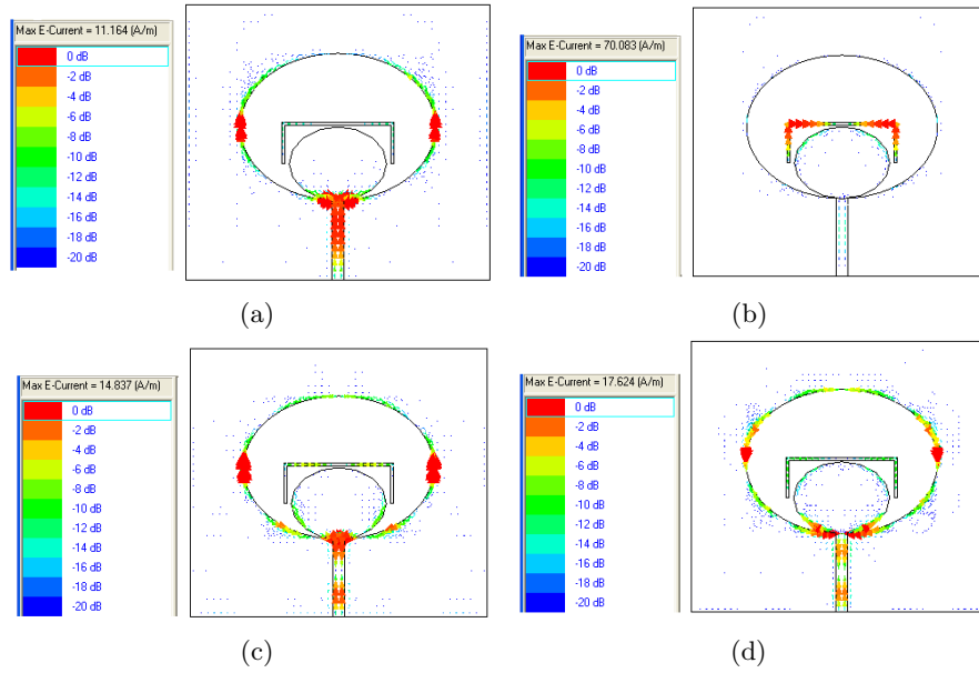
Figure 5. Simulated current distributions of proposed antenna at: (a) 3.5 GHz, (b) 5.15 GHz, (c) 9.0 GHz, and (d) 10.5 GHz.
