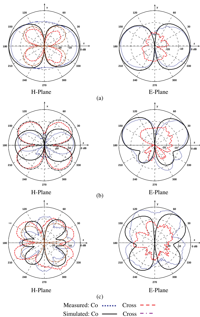
Figure 6. Simulated and measured radiation patterns of proposed antenna at frequencies (a) 4 GHz, (b) 7 GHz, (c) 10 GHz.
