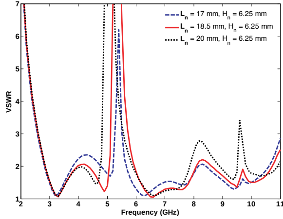
Figure 3. Effects of parameter L_n of the inverted-U strip on the band-notched characteristics of antenna.
