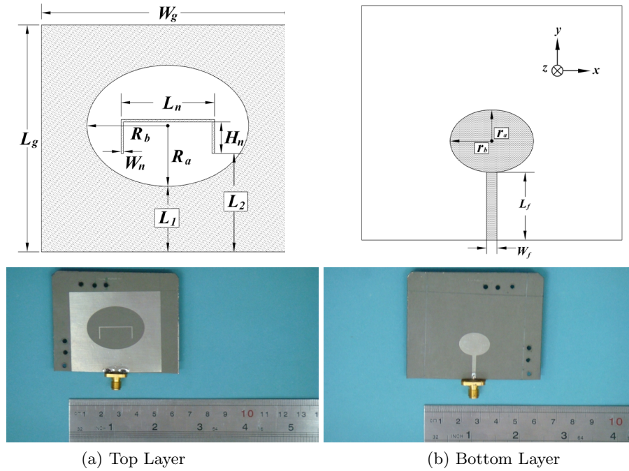
Figure 1. Geometry and photograph of proposed UWB antenna; (a) Elliptical slot with parasitic strip, (b) Feed network.
