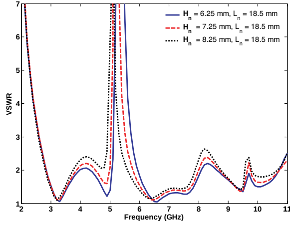
Figure 2. Effects of parameter H_n of the inverted-U strip on the band-notched characteristics of antenna.
