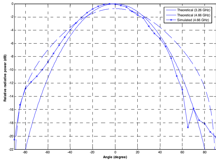
Figure 9. Radiation pattern.
