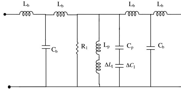
Figure 3. Equivalent circuit of U-slot loaded patch.
