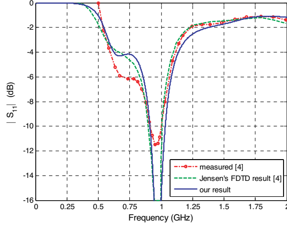
Figure 1. Comparison between the resulting values of |S_{11}| and the results obtained via FDTD technique and the measurements in reference [4] for the \lambda/4 monopole on a PEC handset model.
