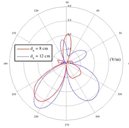
Figure 11. The optimized radiation pattern |E_\theta| of the handset in the presence of the human head at distances ( d_y = 1 cm and d_z = 2 cm).
