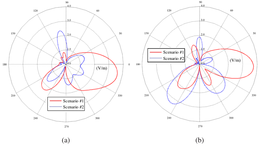
Figure 7. The radiation pattern |E_\theta| of the handset in the presence of the homogeneous human head phantom at distances ( d_y = 1 cm, d_x = 10 cm and d_z = 2 cm). (a) Pre-optimized beampattern, (b) Optimized beampattern.
