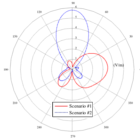
Figure 4. The radiation pattern |E_\theta| for the five-element monopole array mounted on the mobile handset.
