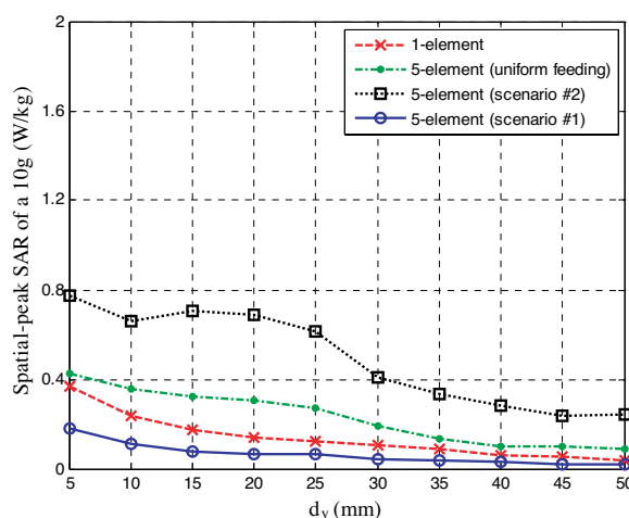
Figure 6. Variation of spatial-peak SAR over 10-g for different distances d_y between handset and outer surface of the homogeneous human head phantom. The handset delivered power is 100 mW.
