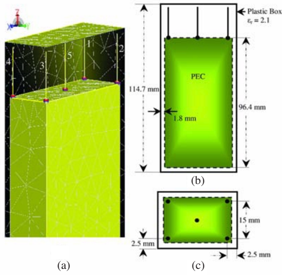
Figure 3. Geometry of the five-element monopole array mounted on the mobile handset. (a) Numerical model, (b) Elevation view, (c) Top view.
