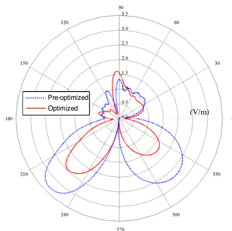
Figure 13. The optimized radiation pattern |E_\theta| of the handset in the presence of the human head at distances ( d_y = 1 cm, d_x = 10 cm and d_z = 4 cm).
