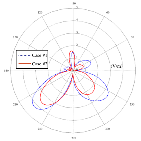
Figure 9. The optimized radiation pattern |E_\theta| of the handset in the presence of the human head at distances ( d_y = 2 cm, d_x = 10 cm and d_z = 2 cm). Cases 1 and 2 are based on re-optimizing the beampattern by exciting the elements with the same amplitude and phase (2, 0^\circ ) or exciting the elements with the previous [Table 5] amplitude and phase, respectively, for the first iteration.
