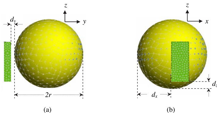
Figure 5. Homogeneous human head model and handset configuration. (a) Front view, (b) Side view.
