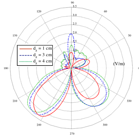
Figure 12. The radiation pattern |E_\theta| of the handset in the presence of the human head for different distances of d_z where d_y = 1 cm and d_x = 10 cm.
