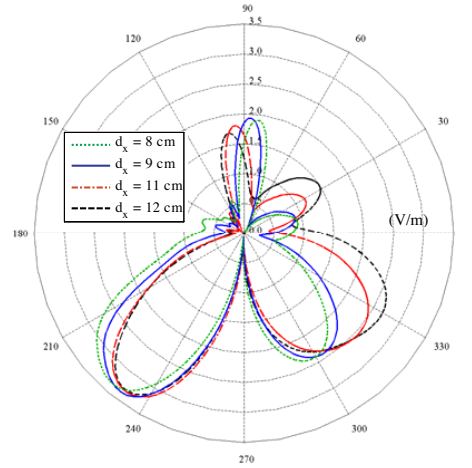
Figure 10. The radiation pattern |E_\theta| of the handset in the presence of the human head for different distances of d_x where d_y = 1 cm and d_z = 2 cm.
