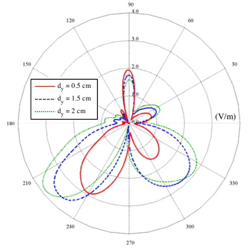
Figure 8. The radiation pattern |E_\theta| of the handset in the presence of the human head for different distances of d_y where d_x = 10 cm and d_z = 2 cm.
