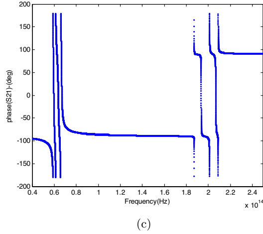
Figure 2. Transmission coefficient (a), reflection coefficient (b), and phase of S21 (c) for N = 5 layers of SRR.
