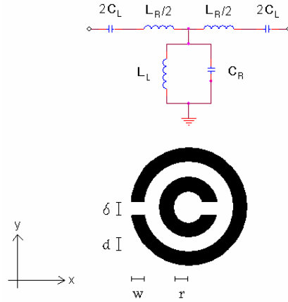
Figure 1. The geometrical feature and equivalent circuit model of the symmetric transmission line of double split ring resonator unit-cell.
