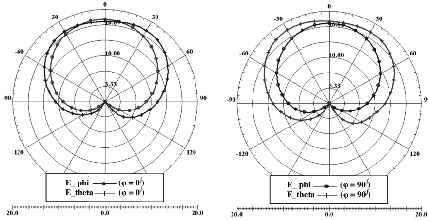
Figure 9. (a) E -plane ( \phi = 0^\circ ) and (b) H -plane ( \phi = 90^\circ ) radiation patterns of the first rectangular dielectric resonator antenna at 2.41 GHz.
