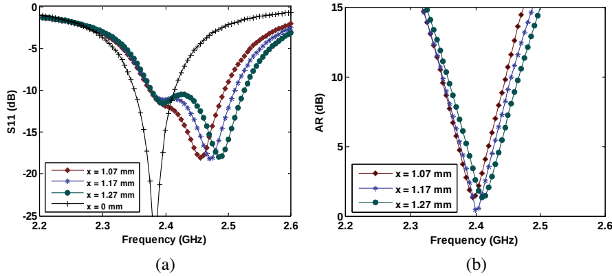
Figure 7. (a) Return loss and (b) axial ratio of the first cylindrical proposed antenna for different values of “ x ” parameter.
