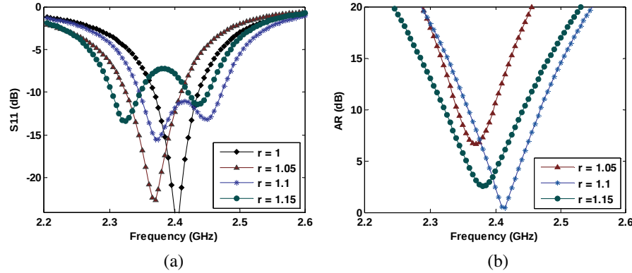
Figure 3. (a) Return loss and (b) axial ratio of the first rectangular antenna for different values of r parameter.
