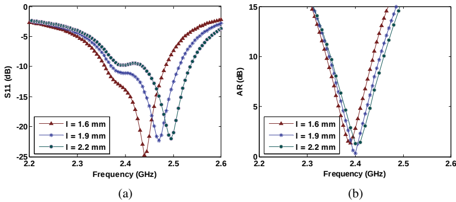
Figure 8. (a) Return loss and (b) axial ratio of the second cylindrical antenna for different values of rectangular notch depth.
