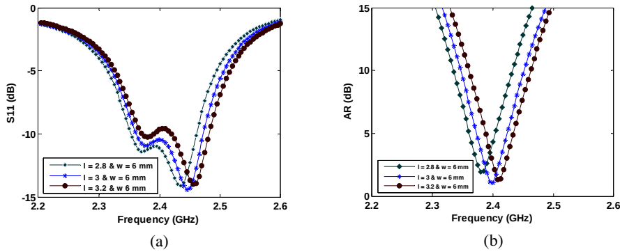
Figure 6. (a) Return loss and (b) axial ratio of the fourth rectangular antenna for different dimensions of perturbation segment.
