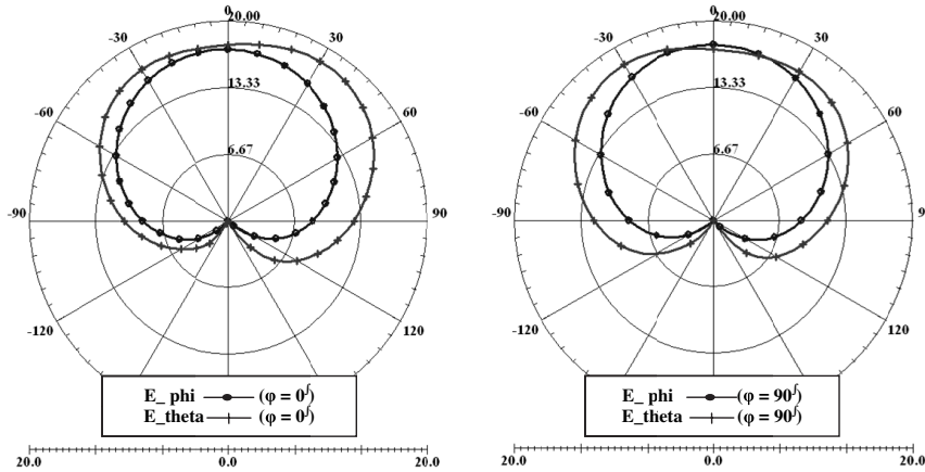
Figure 10. (a) E -plane ( \phi = 0^\circ ) and (b) H -plane ( \phi = 90^\circ ) radiation patterns of the first cylindrical dielectric resonator antenna at 2.40 GHz frequency.
