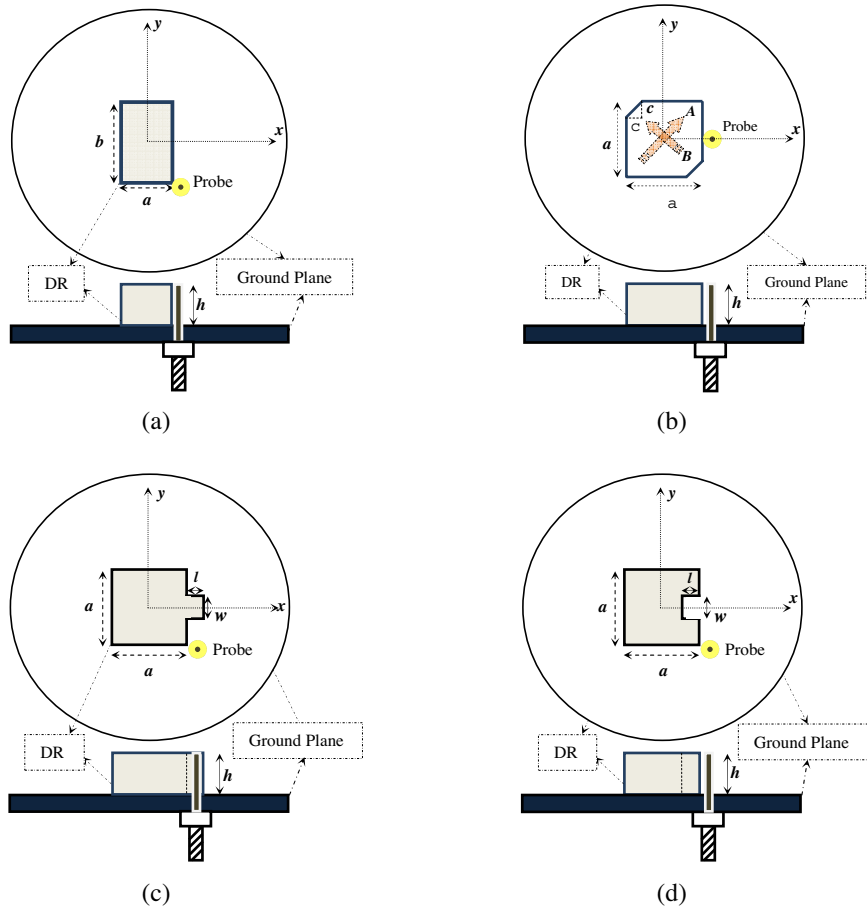
Figure 1. Top and side views of (a) the first, (b) second, (c) third and (d) fourth proposed rectangular DRAs.
