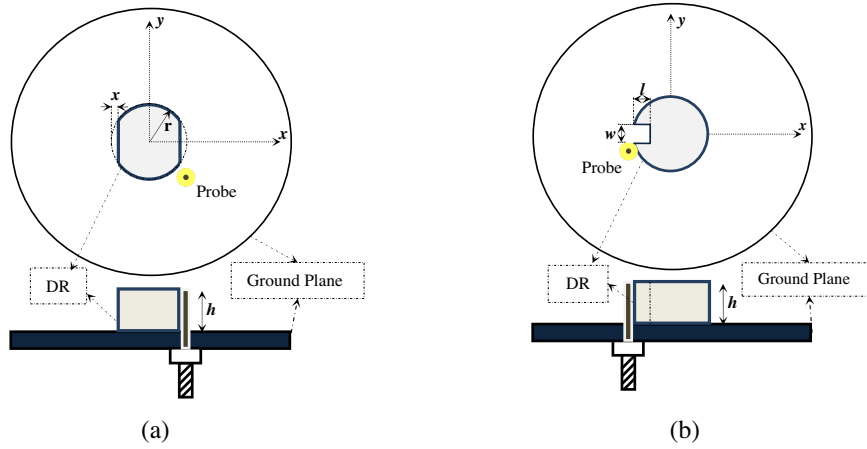
Figure 2. Top and side views of (a) the first and (b) second proposed cylindrical DRAs.
