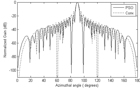
Figure 2. Normalized pattern of 32 element linear array of half wave dipoles. The region of suppressed SLL are [0^\circ, 87^\circ] and [93^\circ, 180^\circ] , and prescribed nulls at 81^\circ and 99^\circ .
