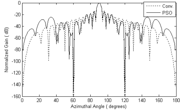
Figure 3. Normalized pattern of 28 element linear array of half wave dipoles. The region of suppressed SLL are [0^\circ, 180^\circ] , and prescribed nulls at 55^\circ , 57.5^\circ , 60^\circ , 120^\circ , 122.5^\circ and 125^\circ .
