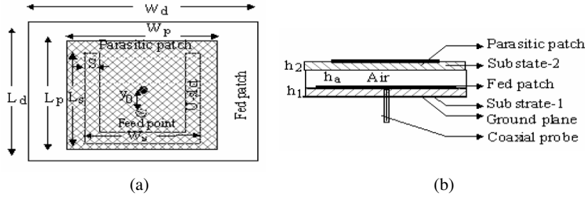
Figure 1. Geometry of the proposed antenna. (a) Top view and (b) side view.
