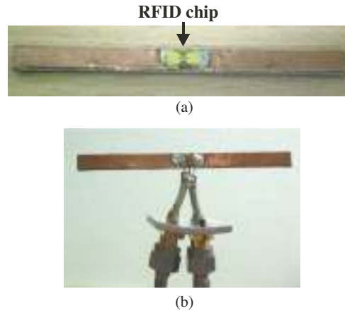
Figure 6. Measurement of a loop tag. (a) A loop antenna for metallic surface, (b) Probing the antenna with the differential probe.
