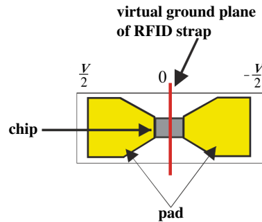
Figure 1. An RFID strap and its virtual ground surface.
