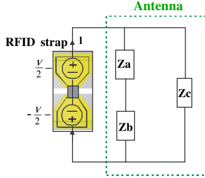
Figure 5. Network model for RFID strap and tag antenna.
