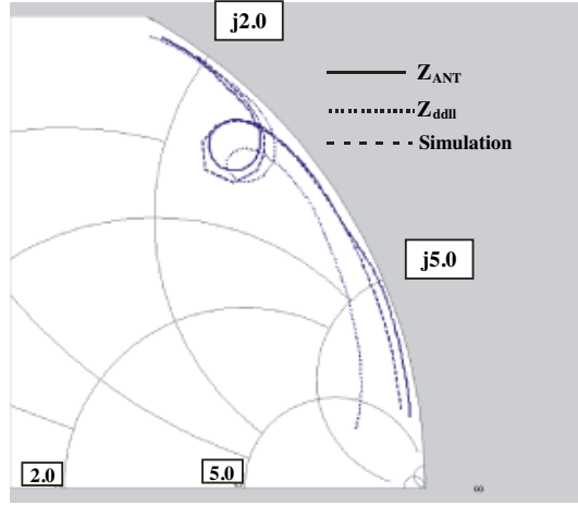
Figure 10. Measurement results of the patch antenna using the differential probe.
