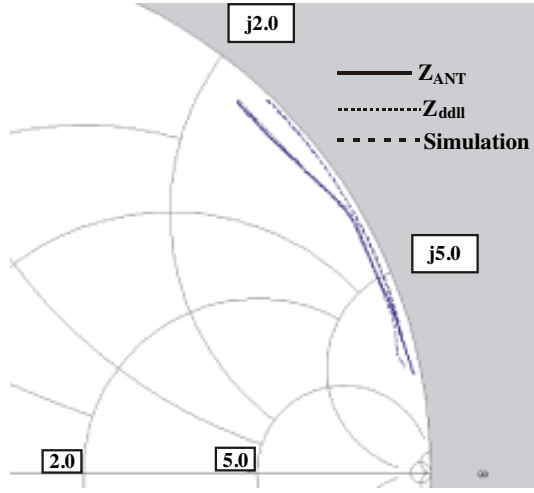
Figure 7. Measurement results of the loop antenna using the differential probe.
