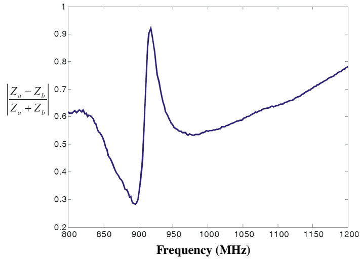
Figure 11. Evaluation of unbalance of the patch antenna.
