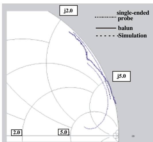
Figure 8. Measurement results of the loop antenna using conventional method.
