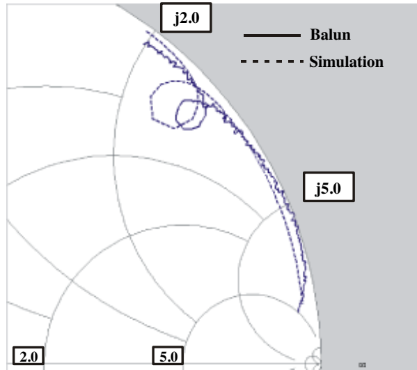
Figure 13. Measurement of the patch antenna using the balun probe.
