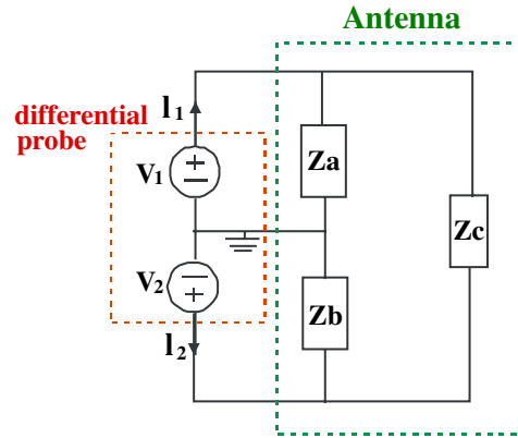
Figure 4. A two-port \pi -network model for the probe and antenna.
