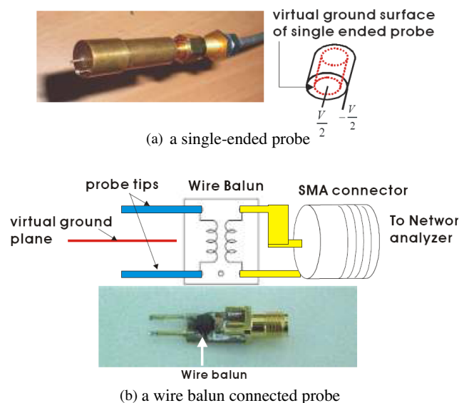
Figure 2. Existing method for RFID tag antenna measurement.
