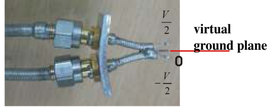
Figure 3. A differential probe and its virtual ground plane.
