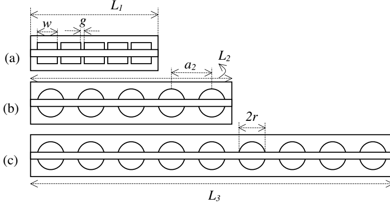
Figure 2. Top view of (a) 5-cell 1-D mushroom-like EBG filter (b) 5-cell circular DGS filter (c) 9-cell circular DGS filter.
