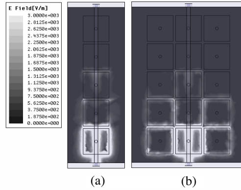
Figure 8. Magnitude of the electric field on the EBG surface for (a) 1-D mushroom-like EBG filter and (b) 2-D mushroom-like EBG filter ( f = 2.4 GHz).
