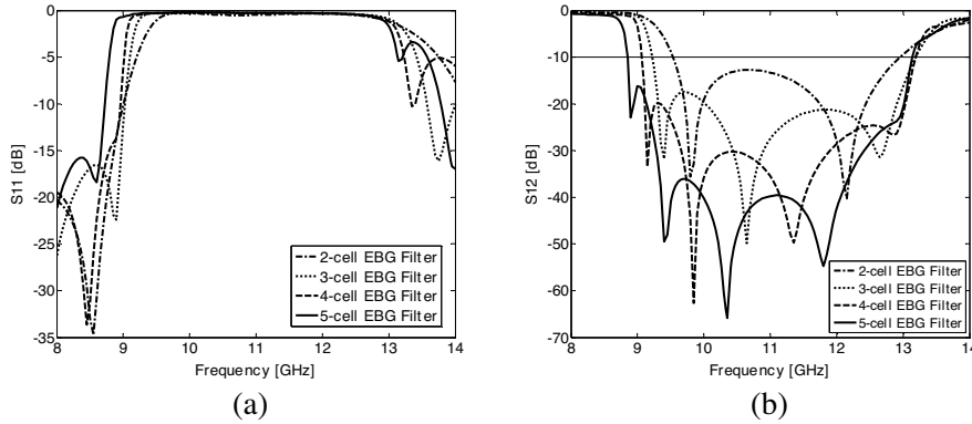
Figure 6. (a) S_{11} and (b) S_{12} parameters of the 1-D EBG filter for various number of EBG cells.
