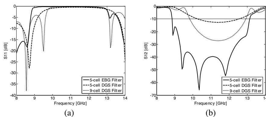
Figure 3. (a) S_{11} and (b) S_{12} parameters of the 1-D 5-cell mushroom-like EBG filter in comparison with 5-cell and 9-cell DGS filters.
