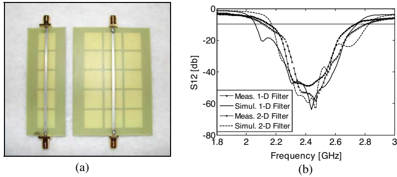
Figure 7. (a) Fabricated 1-D and 2-D mushroom-like EBG filters (b) Measured and simulated S_{12} parameters of 1-D and 2-D EBG filters.
