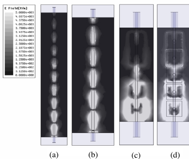
Figure 4. Magnitude of electrical field on the top surface of (a) 9-cell DGS filter (b) 5-cell DGS filter (c) 5-cell mushroom-like EBG filter (d) 5-cell mushroom-like EBG filter on the EBG plane. The scaling factors for (a)–(d) are not the same. f = (12 \text{ GHz}) .
