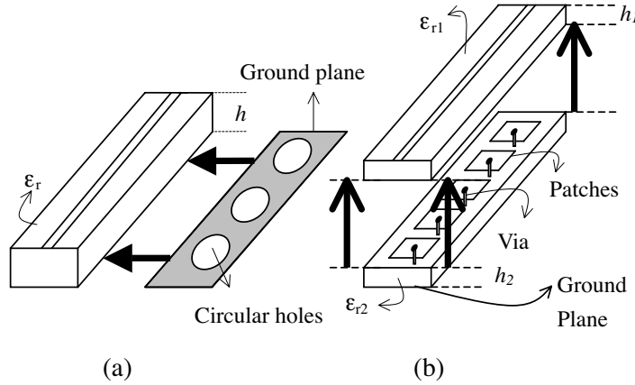
Figure 1. (a) DGS filter with circular holes in the ground (b) 1-D mushroom-like EBG filter.
