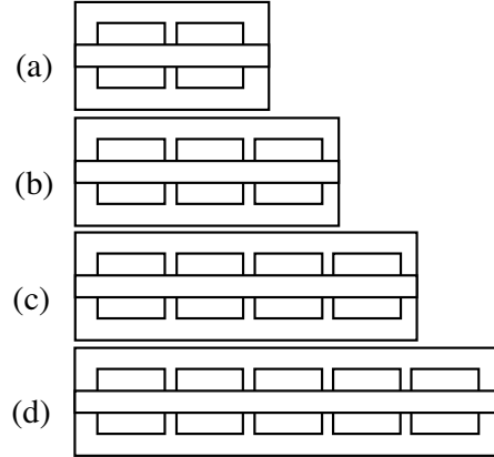
Figure 5. Top view of (a) 2-cell, (b) 3-cell, (c) 4-cell, and (d) 5-cell 1-D mushroom-like EBG filters.
