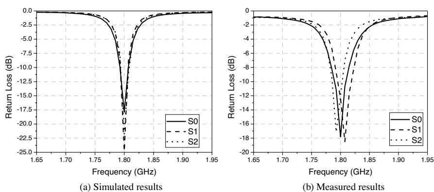
Figure 6. Return losses of the designed small size SCMPAs.
