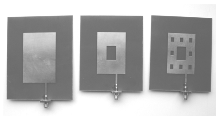
Figure 5. Photograph of the designed edge-fed SCMPAs resonated at 1.8 GHz.
