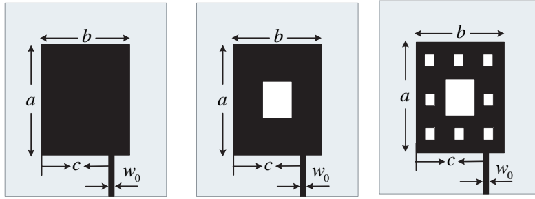
Figure 1. Schematics of the edge-fed Sierpinski carpet microstrip patch antennas of different iteration orders. S0: Zeroth iteration order, S1: First iteration order, S2: Second iteration order.
