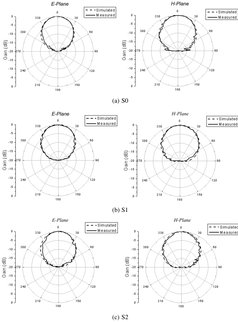
Figure 7. Radiation patterns of the designed small size edge-fed SCMPAs.
