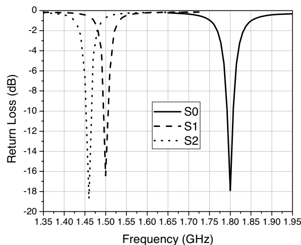
Figure 2. Simulated return losses of the designed edge-fed SCMPAs.
