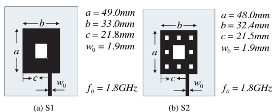
Figure 4. Schematics of designed edge-fed SCMPAs resonated at 1.8 GHz.
