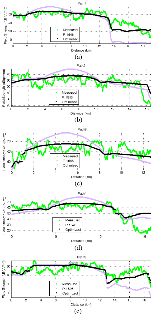
Figure 2. Comparison of the tuned model with the measurements and ITU-R P.1546 for measurement paths.
