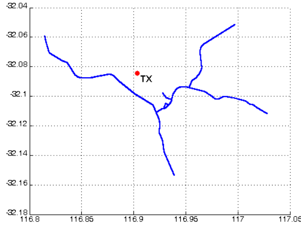
Figure 1. Measurement paths and transmitting antenna location in the longitude-latitude plane.
