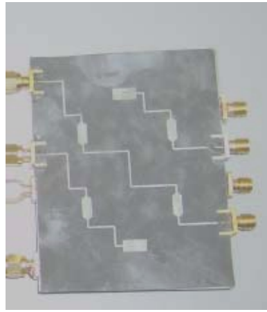
Figure 8. The proposed UWB 4 \times 4 Butler matrix (a) Layout (b) Fabricated.
