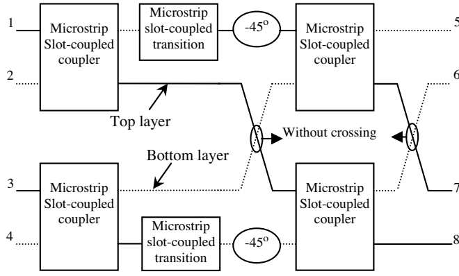
Figure 1. Block diagram of the proposed UWB Butler matrix.
