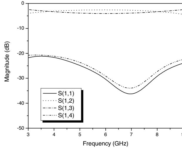
Figure 3. Simulated Scattering parameters of the directional coupler.
