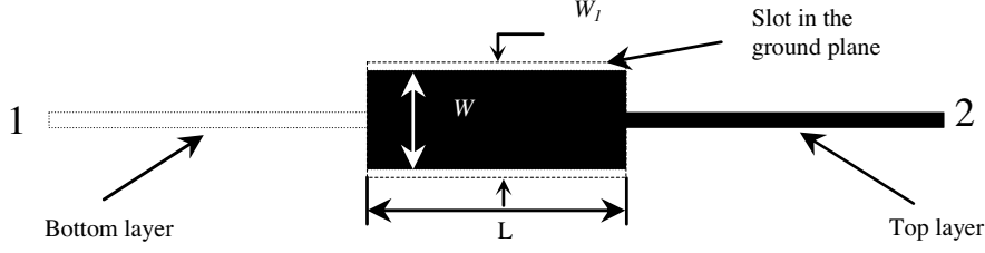
Figure 5. Layout of an improved back-to-back slot coupled transition.
