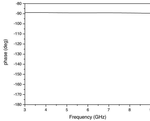
Figure 4. Simulated result of phase shift between the outputs of coupler.
