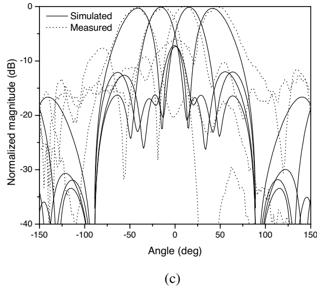
Figure 13. Simulated and measured H -plane radiation pattern (a) 3 GHz (b) 5.8 GHz (c) 9 GHz.
