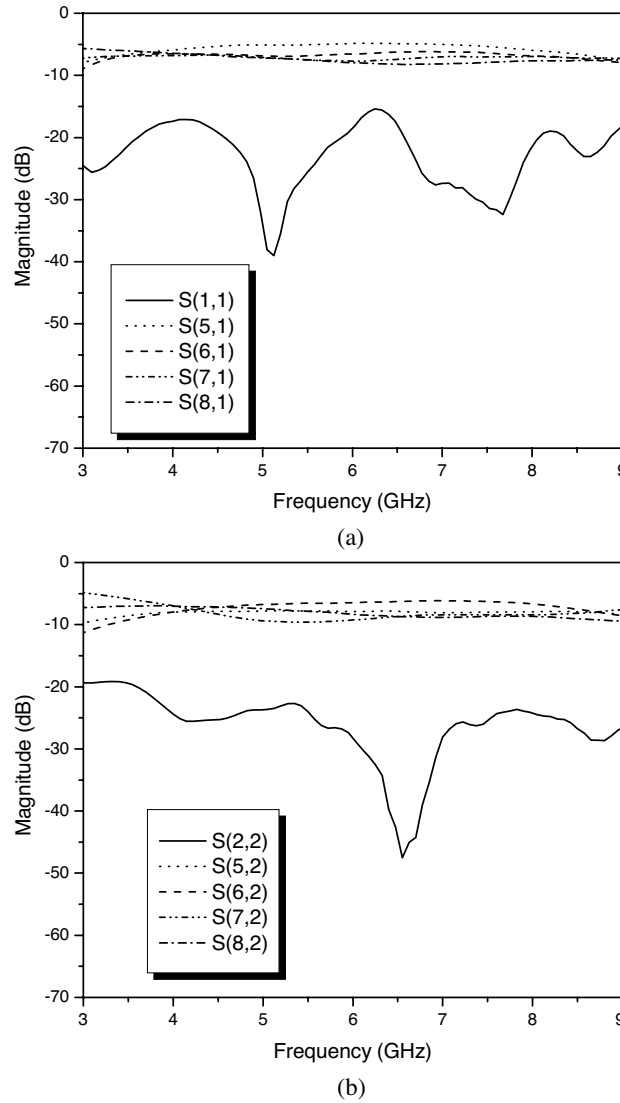
Figure 10. Measured results of the 4X4 Butler matrix (a) Signal at port1 (b) Signal at port2.
