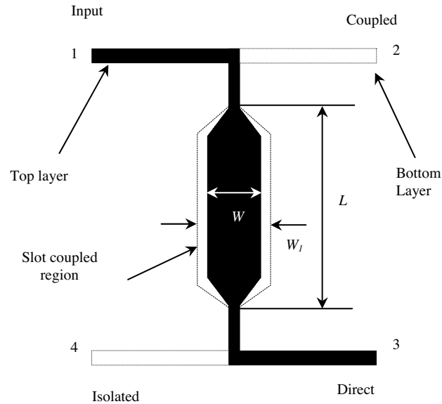
Figure 2. Layout of the microstrip slot-coupled directional coupler.
