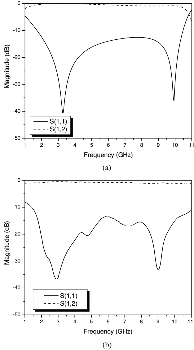
Figure 7. Scattering parameters of the transition: (a) Simulated, (b) Measured.
