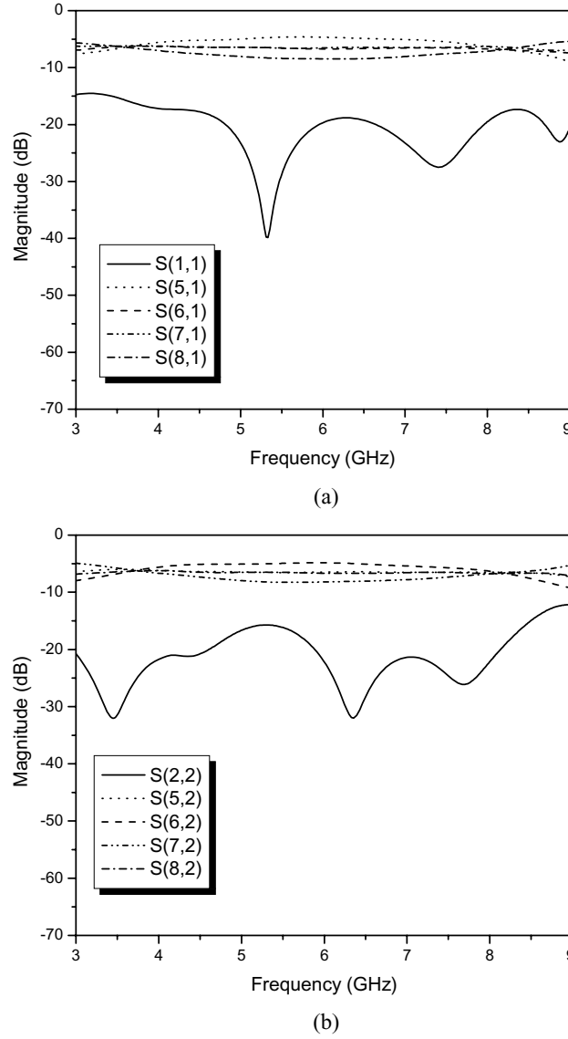
Figure 9. Simulated results of the 4 \times 4 Butler matrix (a) Signal at port1 (b) Signal at port2.
