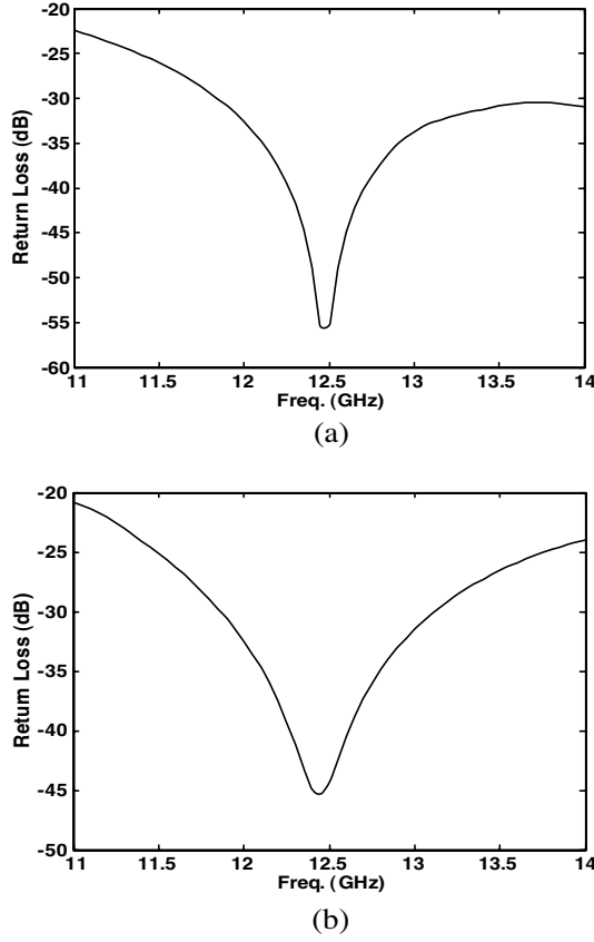
Figure 11. Frequency characteristics of coax gap adaptor with (a) h_2 = 9.6 mm and (b) h_2 = 6 mm, f_0 = 12.45 GHz, d_{in} = 1.3 mm, d_{out} = 3.3 mm, \epsilon_r = 2.1 .
