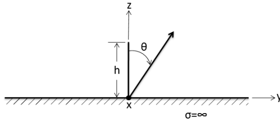
Figure 3. Monopole on infinite electric conductor.
