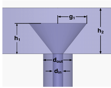
Figure 8. Conical probe adaptor.
