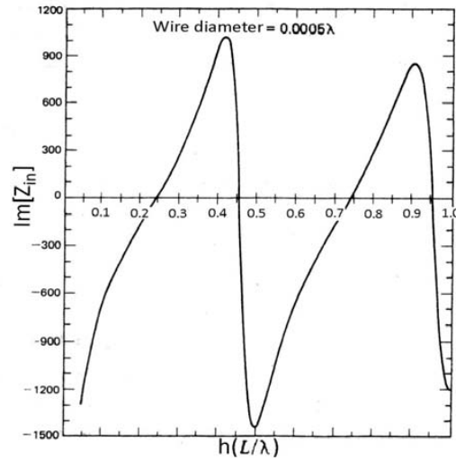
Figure 4. Calculated input reactance for monopole antenna as antenna height, h [21].
