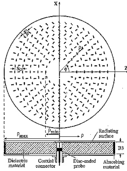
Figure 1. A radial line slot antenna with linear polarization and coax gap to radial line adaptor [1].
