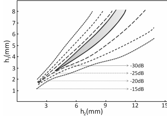
Figure 10. Return loss of conical feed as function of h_1 and h_2 for optimized g_1 , f_0 = 12.45 GHz, d_{in} = 1.3 mm, d_{out} = 3.3 mm, \epsilon_r = 2.1 .
