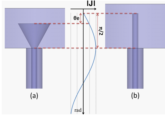
Figure 9. Current distribution on conventional and conical probes.
