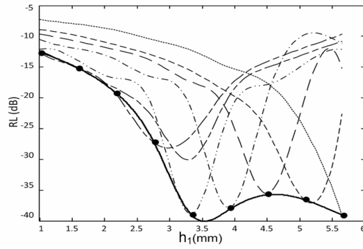
Figure 16. Effect of changing h_1 when other parameters are fixed, on RL.
