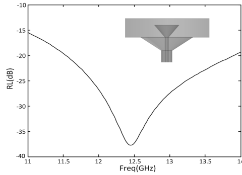
Figure 17. Reflection characteristics of a funnel probe adaptor. f_0 = 12.45 GHz, h_1 = 3.6 mm, h_2 = \lambda/4 , g_2 = \lambda/2 , h_3 = 12.2 mm, g_1 = 2.9 mm.
