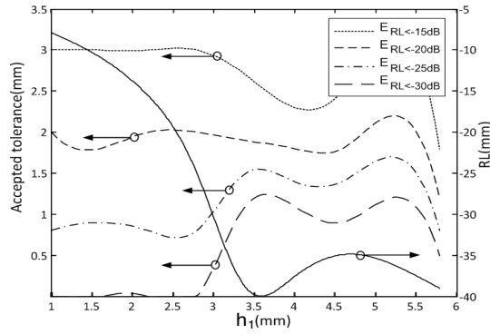
Figure 15. Acceptable tolerance for reflections below -15 dB, -20 dB, -25 dB and -30 dB and optimized reflection as a function of h_1 .
