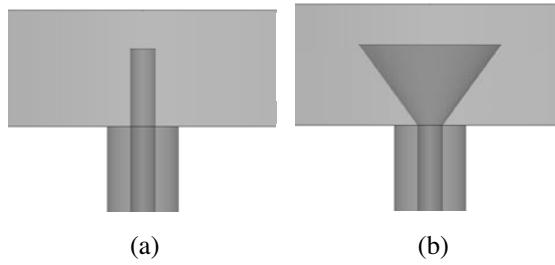
Figure 2. RLSA antenna adapters (a) conventional (b) conical probe.
