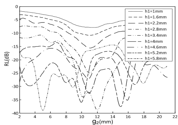
Figure 13. Reflection from funnel probe adaptor as a function of g_2 for various h_1 .
