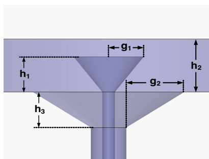
Figure 12. Funnel probe adaptor.
