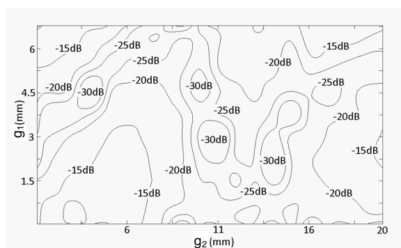
Figure 14. Reflection from funnel probe adaptor as functions of g_2 and g_1 .
