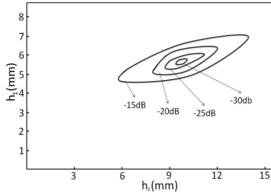
Figure 6. Return loss of the probe as function of h_1 and h_2 , d_{in} = 1.3 mm, d_{out} = 3.3 mm, \varepsilon_r = 2.1 .
