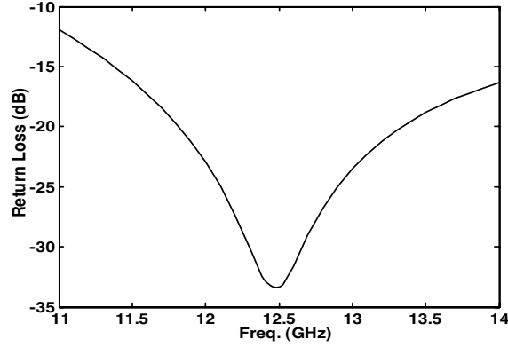
Figure 7. The frequency characteristics of coax gap adaptor with h_1 = 5.4 mm and h_2 = 9.6 mm.
