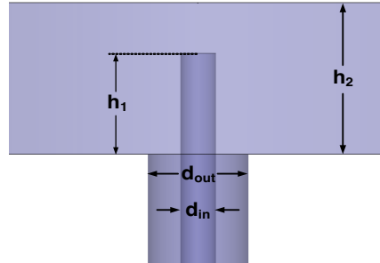
Figure 5. Conventional probe adaptor for f_0 = 12.45 GHz, d_{in} = 1.3 mm, d_{out} = 3.3 mm, \epsilon_r = 2.1 .
