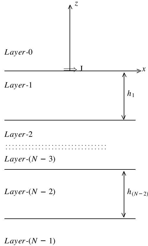
Figure 1. A current source in a multilayered medium.
