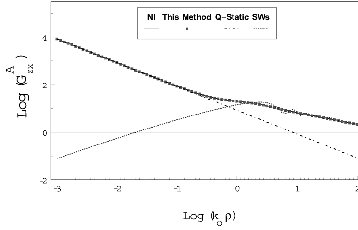
Figure 4. Magnitude of G_{zx}^A in a four-layered medium: Layer 0: air, layer 1: h_1 = 1.5 mm, \epsilon_{r1} = 2 , layer 2: h_2 = 0.75 mm, \epsilon_{r2} = 10 , layer 3: PEC. z' = z = 0 . f = 15 GHz.
