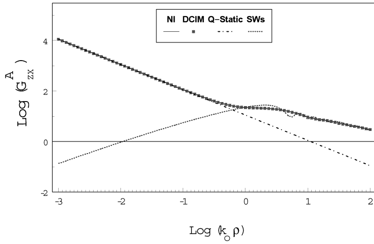
Figure 5. Magnitude of G_{zx}^A in a four-layered medium: Layer 0: air, layer 1: h_1 = 1.5 mm, \epsilon_{r1} = 2 , layer 2: h_2 = 0.75 mm, \epsilon_{r2} = 10 , layer 3: PEC. z' = z = 0 . f = 20 GHz.
