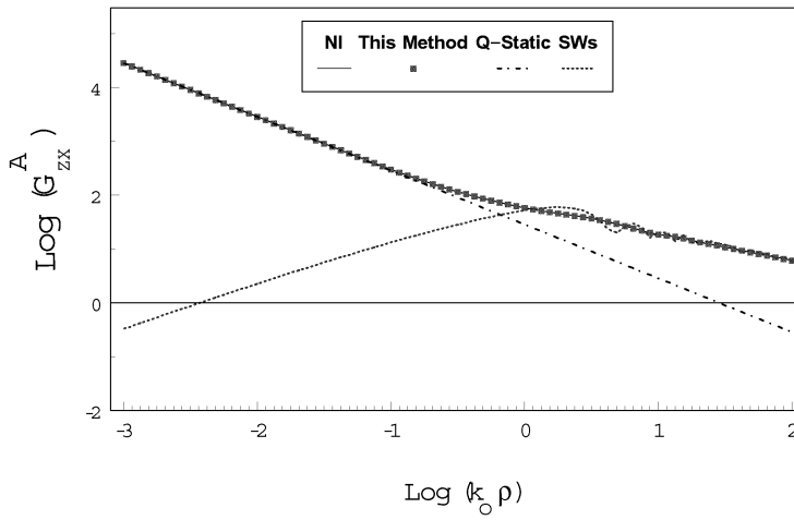
Figure 3. Magnitude of G^A_{zx} in a three-layered medium: Layer 0: air, layer 1: h_1 = 1.0 mm, \epsilon_{r1} = 12.6 , layer 2: PEC. z' = z = 0 . f = 20 GHz.
