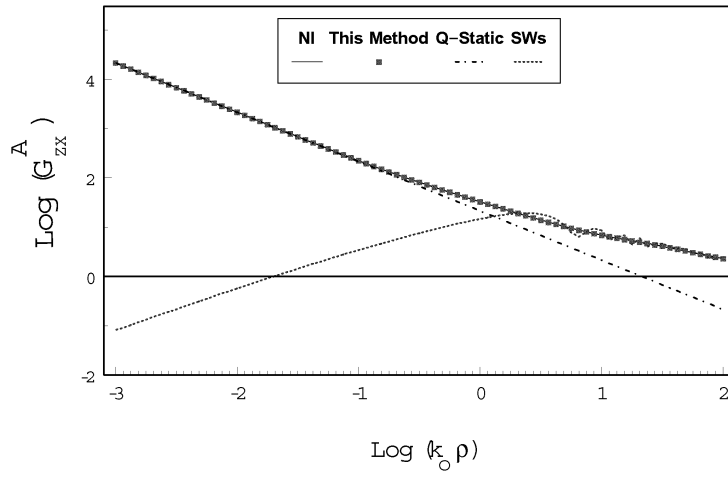
Figure 2. Magnitude of G^A_{zx} in a three-layered medium: Layer 0: air, layer 1: h_1 = 1.0 mm, \epsilon_{r1} = 12.6 , layer 2: PEC. z' = z = 0 . f = 15 GHz.
