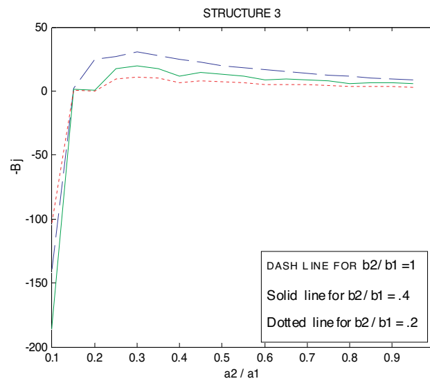
Figure 6. Susceptance verses step ratio for the 3D step.
