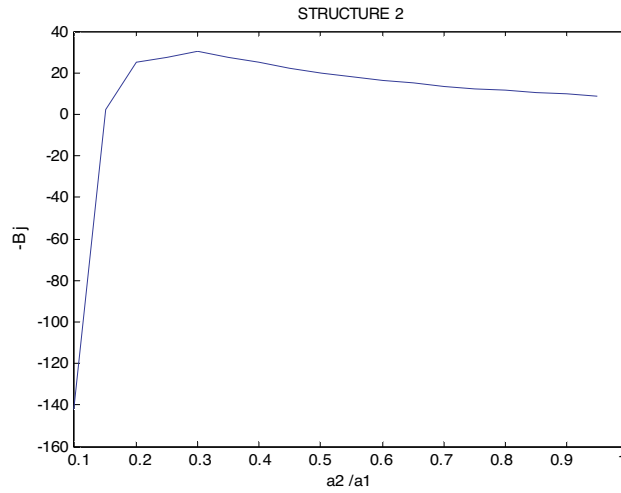
Figure 5. Susceptance verses step ratio for the x -directed step.
