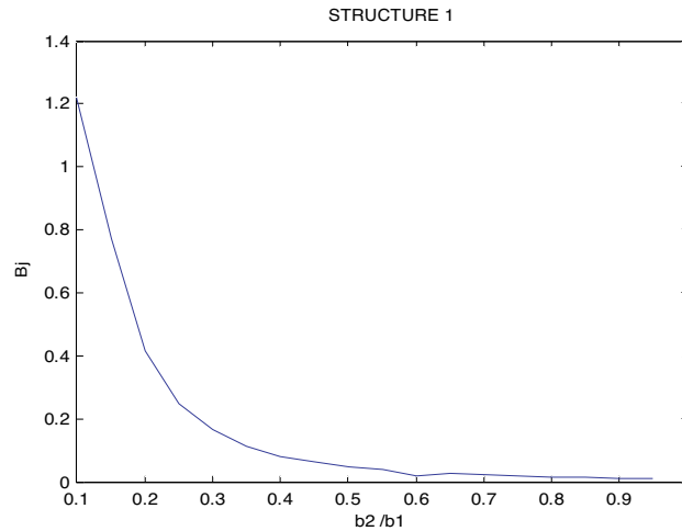
Figure 4. Susceptance verses step ratio for the y -directed step.
