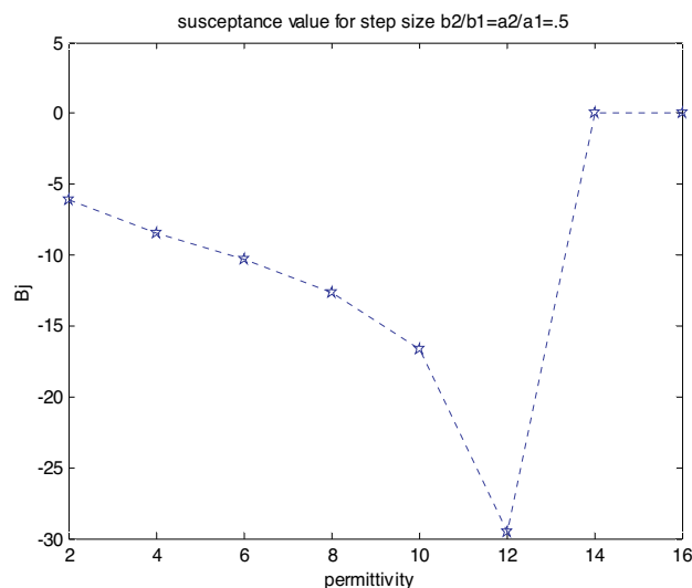
Figure 7. Susceptance verses permittivity for step size ( a_2/a_1 = b_2/b_1 = .5 ).
