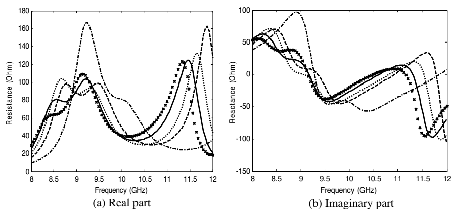
Figure 15. The input impedance corresponding to best axial ratio of Figure 13.
