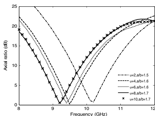
Figure 8. The best axial ratio of superquadric DRA at different squariness parameter.
