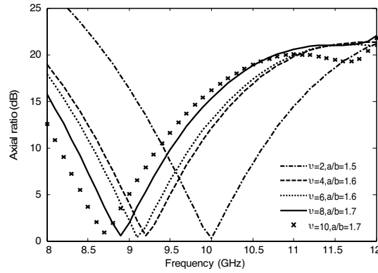
Figure 13. The best axial ratio of superquadric DRA at different squareness parameter.
