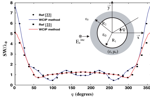
Figure 9. Plots of the normalized SW versus the observation angle of a single conducting cylinder coated with either dielectric or metamaterial.
