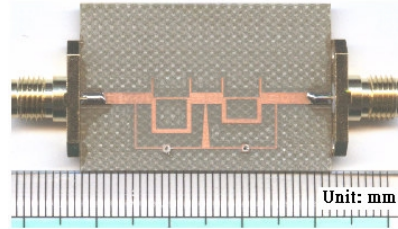
Figure 6. Photograph of a fabricated broadband bandpass filter.
