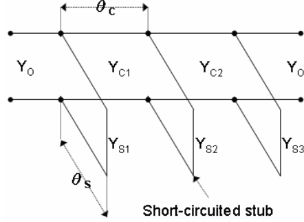
Figure 2. Circuit model for a pseudo distributed bandpass filter with three short-circuited stubs.
