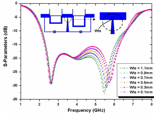
Figure 4. Simulated magnitude of S_{11} (dB) for the broadband bandpass filter in different width of the tapped stub ( W_{ts} ).
