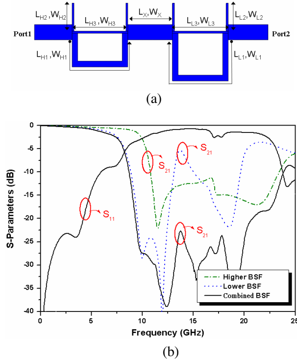
Figure 3. (a) Geometry and (b) simulated S -Parameters of the combined bandstop filter consists of higher BSF and lower BSF.
