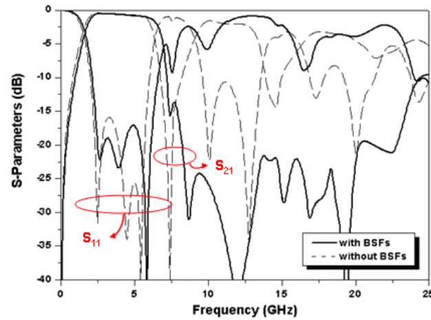
Figure 5. Simulated S -parameters of the proposed broadband bandpass filter with/without BSFs.
