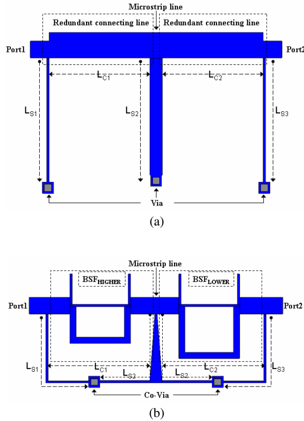
Figure 1. Geometry of (a) the traditional broadband BPF and (b) the proposed branch stubs co-via broadband bandpass filter with combined BSF substituted for redundant connecting lines.
