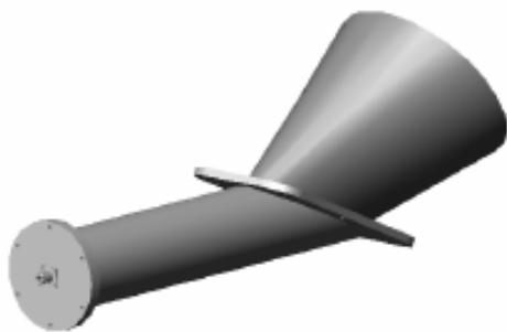
Figure 16. Fabricated Vlasov antenna equipped with circular Horn.
