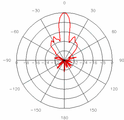
Figure 8. Half Power Beam Width for H -plane (\text{HPBW})_H = 11^\circ .
