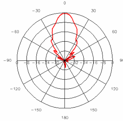
Figure 15. Half Power Beam Width (HPBW)_H = 16^\circ .
