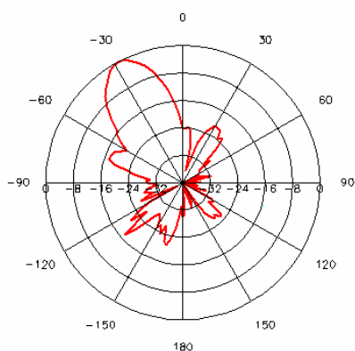
Figure 7. Half Power Beam Width for E -plane (\text{HPBW})_E = 17^\circ .
