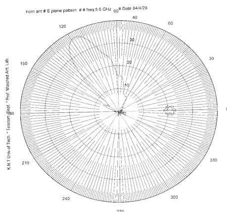
Figure 17. E -plane pattern of Horn antenna, (\text{HPBW})_E = 13.7^\circ at frequency f = 5.6 GHz.
