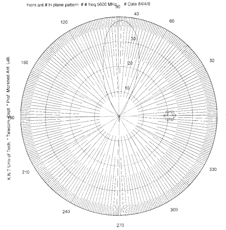
Figure 18. H -plane pattern of Horn antenna, (\text{HPBW})_H = 16.2^\circ at frequency f = 5.6 \text{ GHz} .
