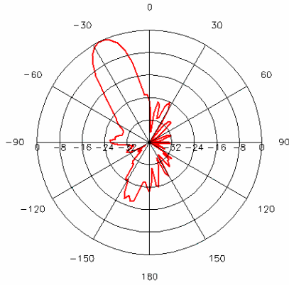
Figure 14. Half Power Beam Width (HPBW)_E = 13^\circ .
