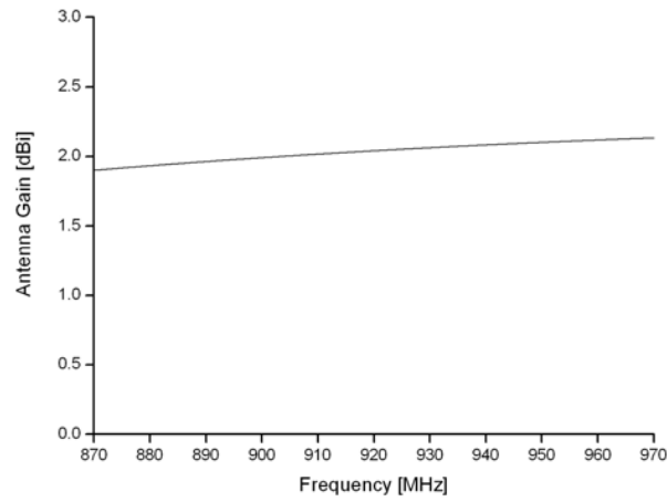
Figure 7. Measured gain of the proposed antenna.
