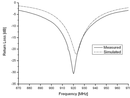
Figure 3. Measured and simulated return losses of the proposed antenna.
