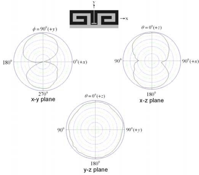
Figure 6. Measured radiation patterns at 922 MHz for the proposed antenna.
