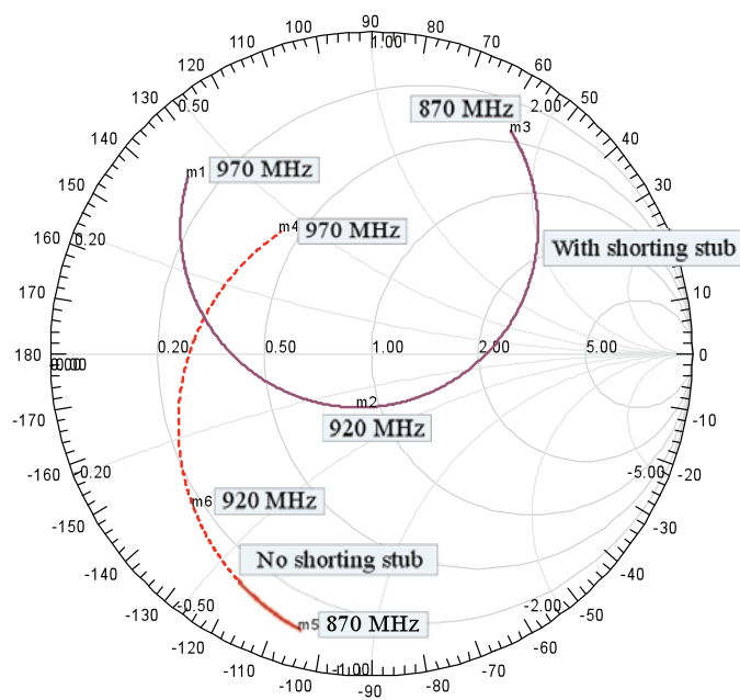
Figure 5. The impedance variation with shorting stub and no shorting stub.
