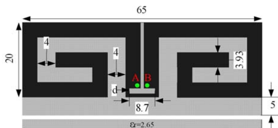
Figure 1. Geometry of the proposed printed dipole antenna.
