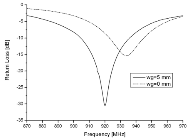
Figure 4. Return losses for the proposed antenna when wg = 5 mm and wg = 0 mm.
